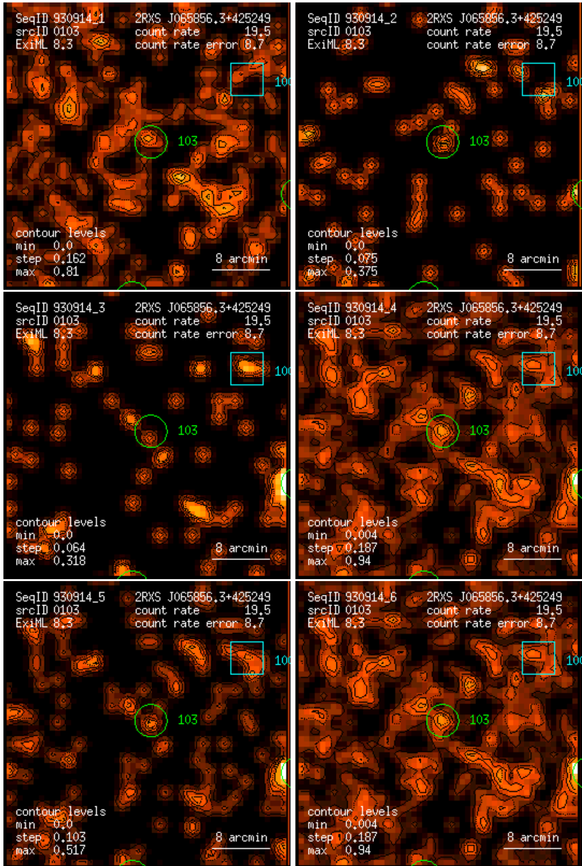
Figure 103: RASS 930914: detection 0103: band rate images, Gaussian filter: (1) PSPC channels 11 – 41, (2) 52 – 90, (3) 91 – 201, (4) 11 – 235, (5) 52 – 201, (6) 11 – 201. Broad band rates in counts/ks. Band rate contour levels in counts/ks/arcmin 2 .
