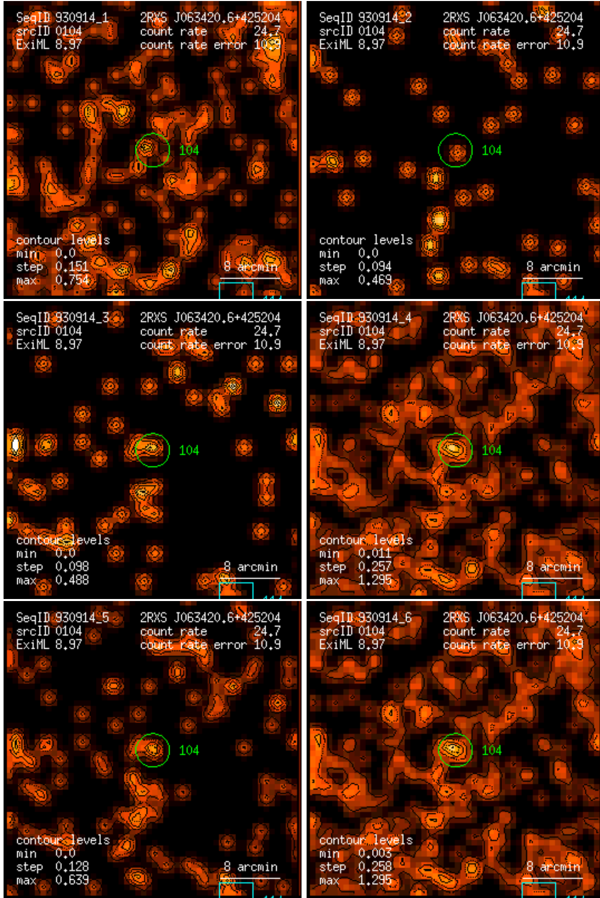
Figure 104: RASS 930914: detection 0104: band rate images, Gaussian filter: (1) PSPC channels 11 – 41, (2) 52 – 90, (3) 91 – 201, (4) 11 – 235, (5) 52 – 201, (6) 11 – 201. Broad band rates in counts/ks. Band rate contour levels in counts/ks/arcmin 2 .
