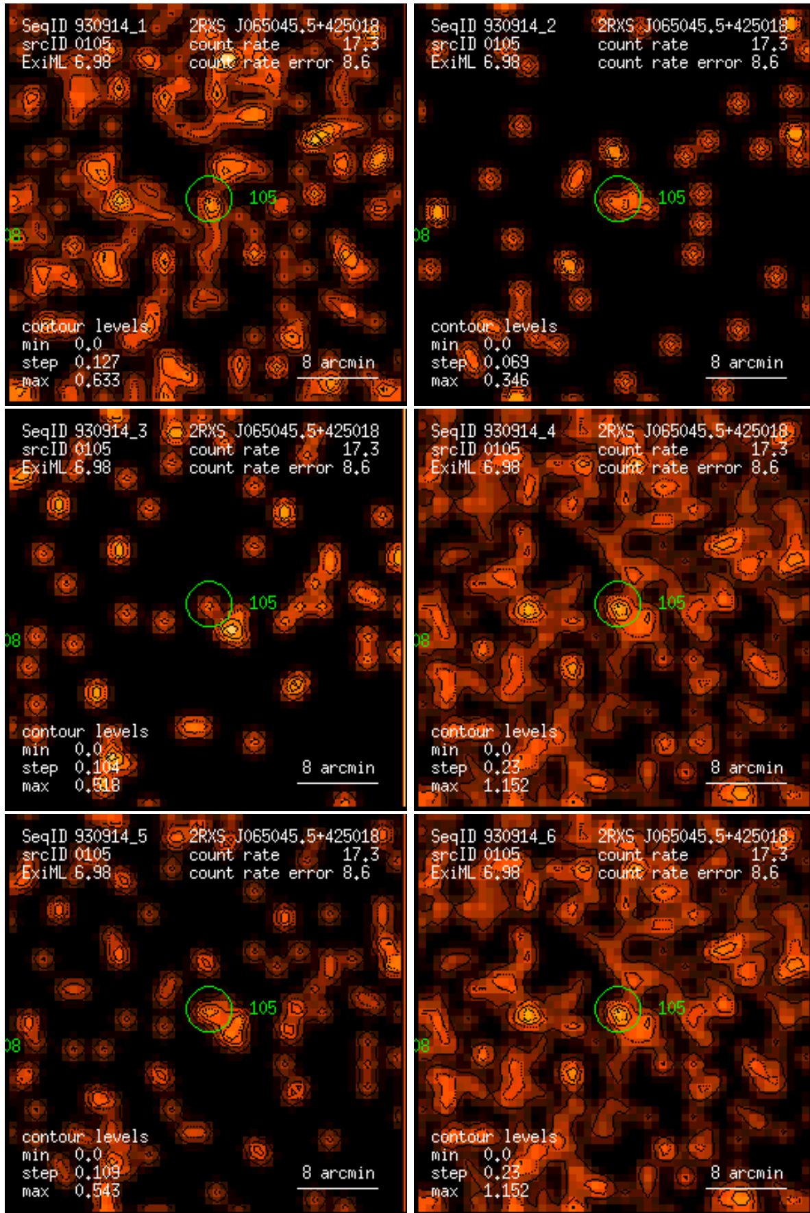
Figure 105: RASS 930914: detection 0105: band rate images, Gaussian filter: (1) PSPC channels 11 – 41, (2) 52 – 90, (3) 91 – 201, (4) 11 – 235, (5) 52 – 201, (6) 11 – 201. Broad band rates in counts/ks. Band rate contour levels in counts/ks/arcmin 2 .
