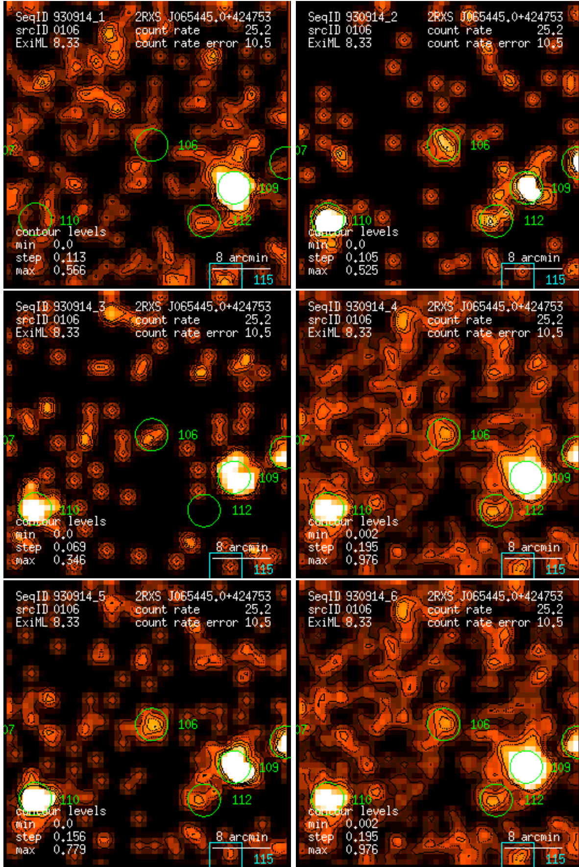
Figure 106: RASS 930914: detection 0106: band rate images, Gaussian filter: (1) PSPC channels 11 – 41, (2) 52 – 90, (3) 91 – 201, (4) 11 – 235, (5) 52 – 201, (6) 11 – 201. Broad band rates in counts/ks. Band rate contour levels in counts/ks/arcmin 2 .
