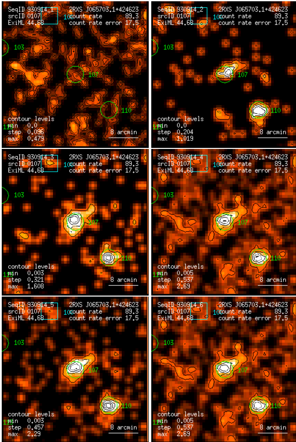
Figure 107: RASS 930914: detection 0107: band rate images, Gaussian filter: (1) PSPC channels 11 – 41, (2) 52 – 90, (3) 91 – 201, (4) 11 – 235, (5) 52 – 201, (6) 11 – 201. Broad band rates in counts/ks. Band rate contour levels in counts/ks/arcmin 2 .
