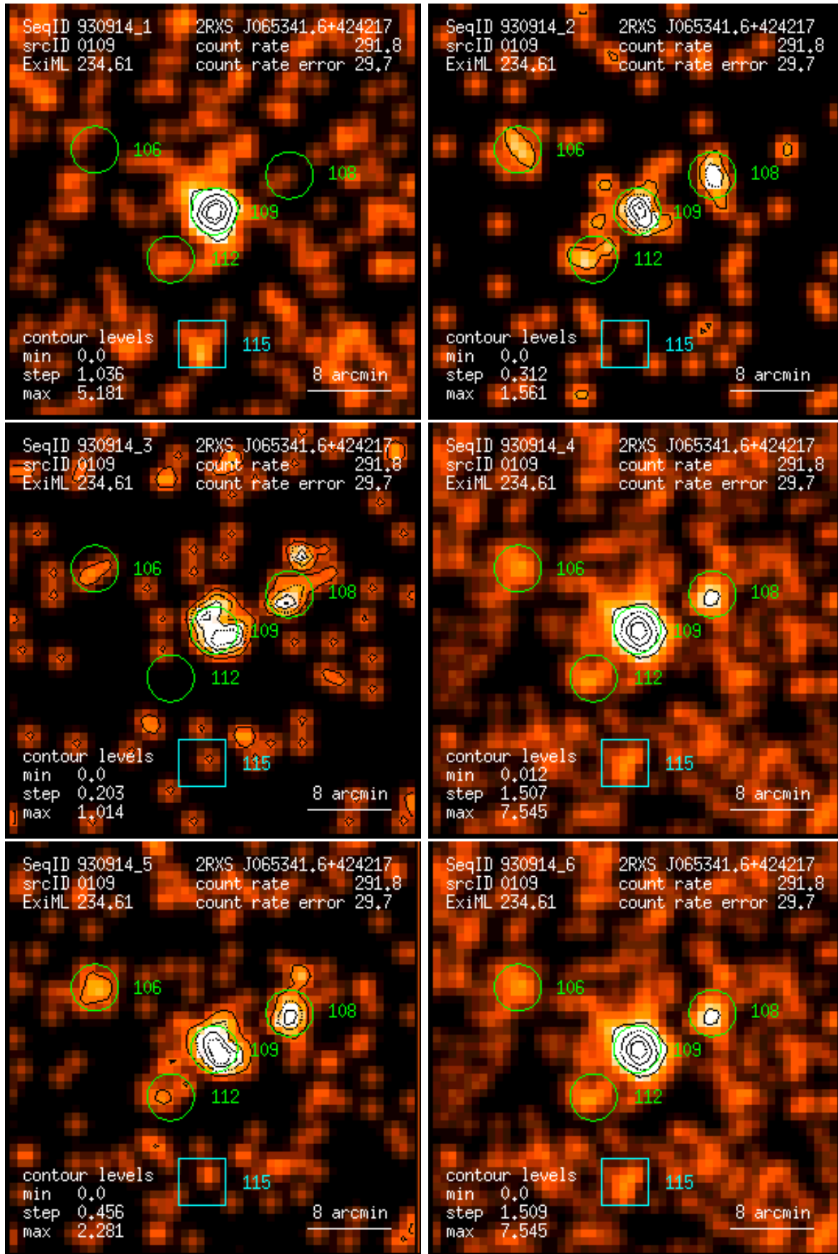
Figure 109: RASS 930914: detection 0109: band rate images, Gaussian filter: (1) PSPC channels 11 – 41, (2) 52 – 90, (3) 91 – 201, (4) 11 – 235, (5) 52 – 201, (6) 11 – 201. Broad band rates in counts/ks. Band rate contour levels in counts/ks/arcmin 2 .
