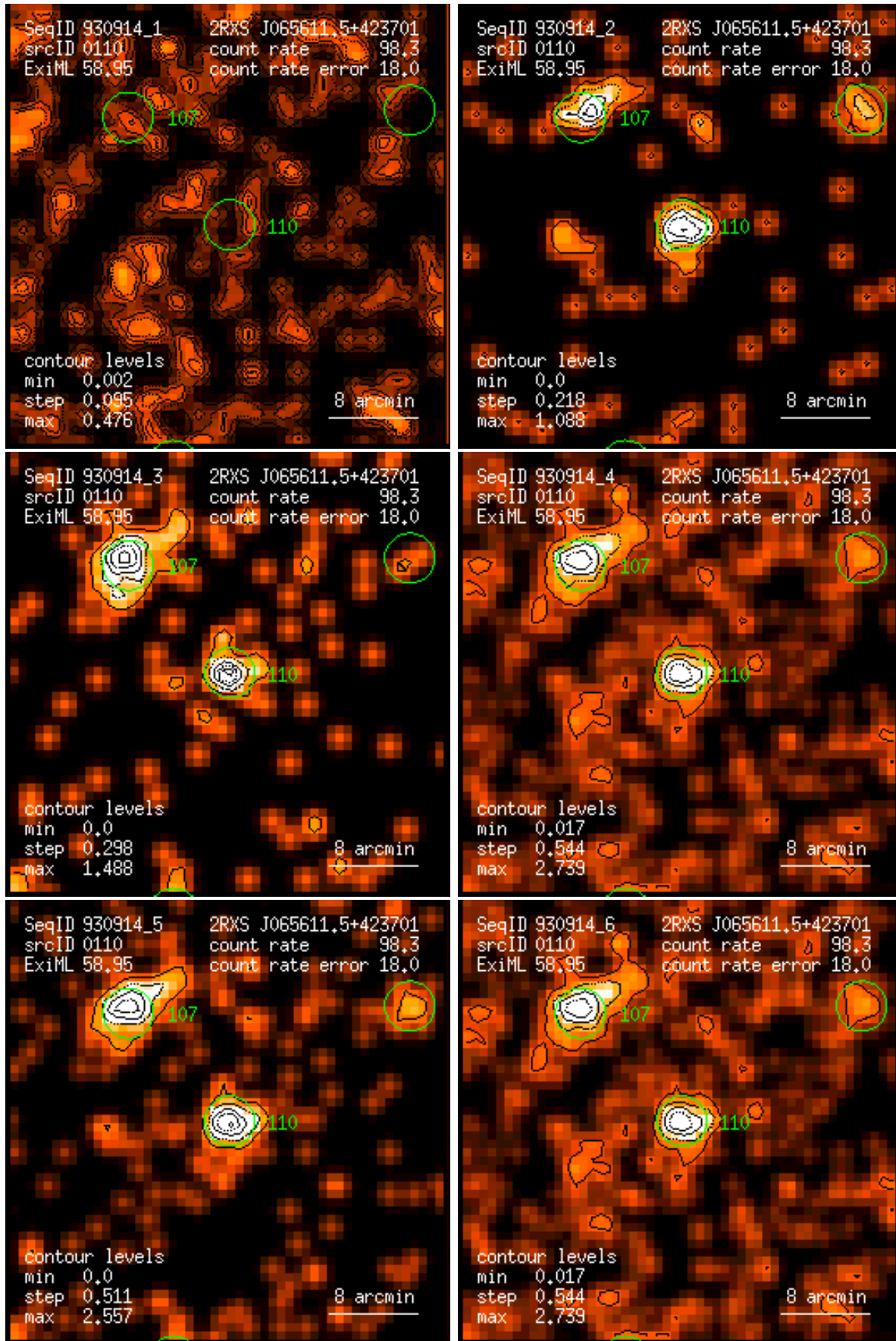
Figure 110: RASS 930914: detection 0110: band rate images, Gaussian filter: (1) PSPC channels 11 – 41, (2) 52 – 90, (3) 91 – 201, (4) 11 – 235, (5) 52 – 201, (6) 11 – 201. Broad band rates in counts/ks. Band rate contour levels in counts/ks/arcmin 2 .
