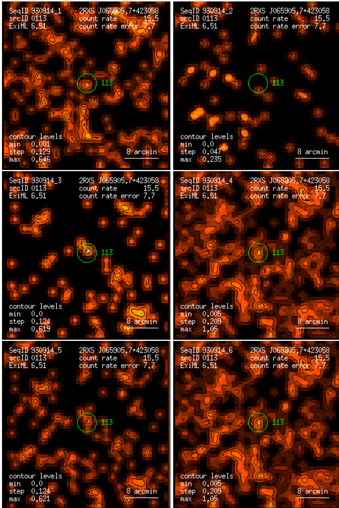
Figure 113: RASS 930914: detection 0113: band rate images, Gaussian filter: (1) PSPC channels 11 – 41, (2) 52 – 90, (3) 91 – 201, (4) 11 – 235, (5) 52 – 201, (6) 11 – 201. Broad band rates in counts/ks. Band rate contour levels in counts/ks/arcmin 2 .
