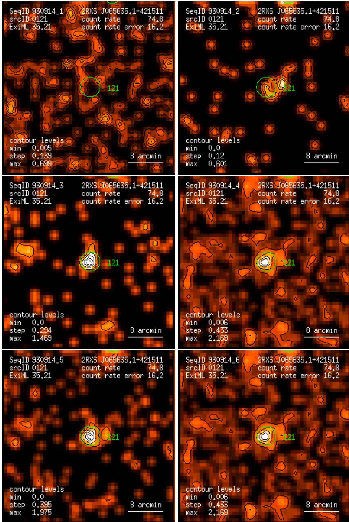
Figure 121: RASS 930914: detection 0121: band rate images, Gaussian filter: (1) PSPC channels 11 – 41, (2) 52 – 90, (3) 91 – 201, (4) 11 – 235, (5) 52 – 201, (6) 11 – 201. Broad band rates in counts/ks. Band rate contour levels in counts/ks/arcmin 2 .
