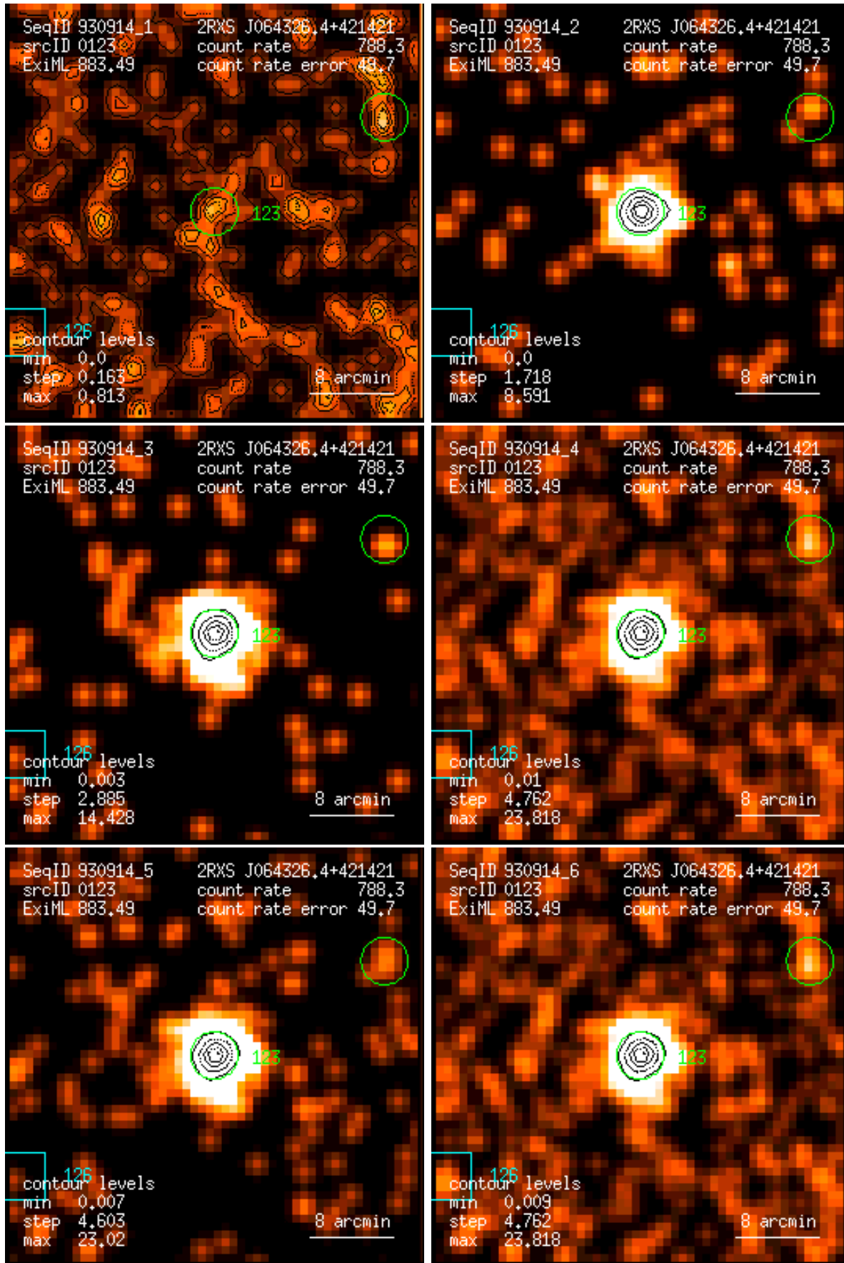
Figure 123: RASS 930914: detection 0123: band rate images, Gaussian filter: (1) PSPC channels 11 – 41, (2) 52 – 90, (3) 91 – 201, (4) 11 – 235, (5) 52 – 201, (6) 11 – 201. Broad band rates in counts/ks. Band rate contour levels in counts/ks/arcmin 2 .
