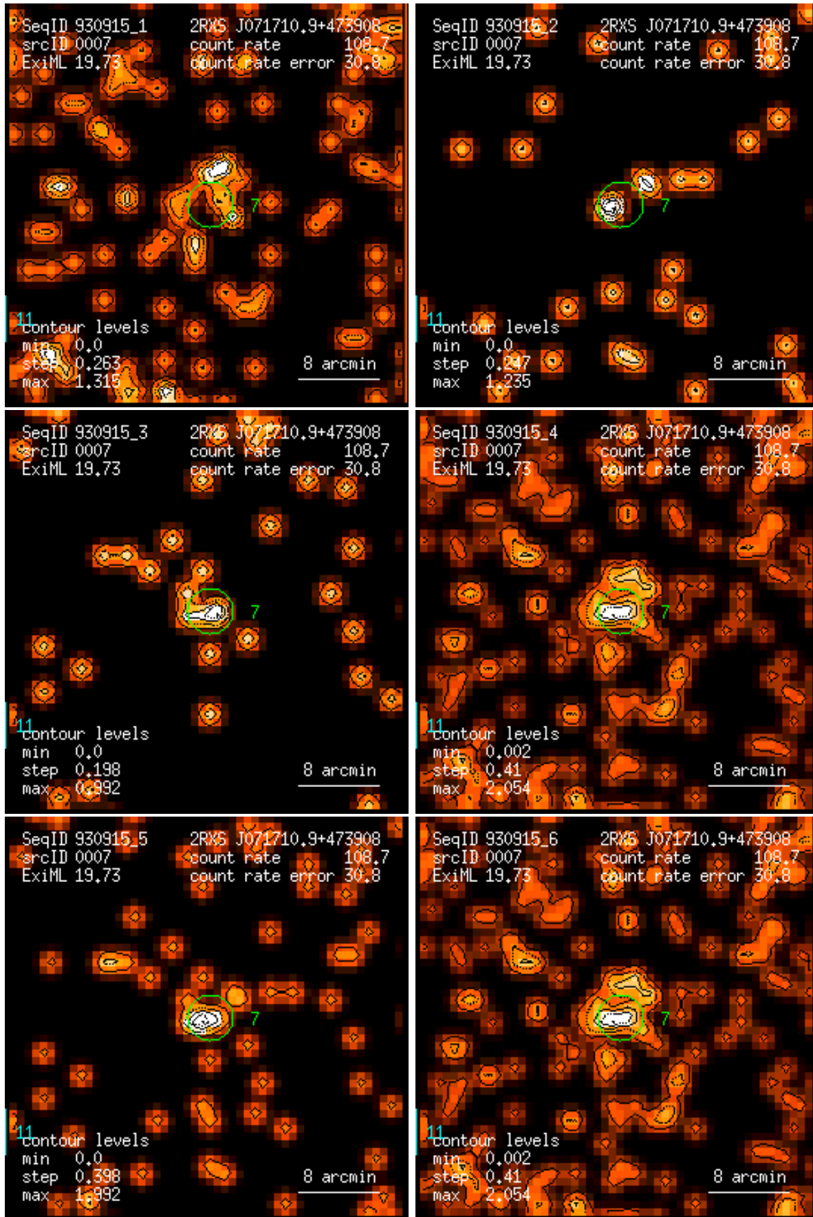
Figure 7: RASS 930915: detection 0007: band rate images, Gaussian filter: (1) PSPC channels 11 – 41, (2) 52 – 90, (3) 91 – 201, (4) 11 – 235, (5) 52 – 201, (6) 11 – 201. Broad band rates in counts/ks. Band rate contour levels in counts/ks/arcmin 2 .
