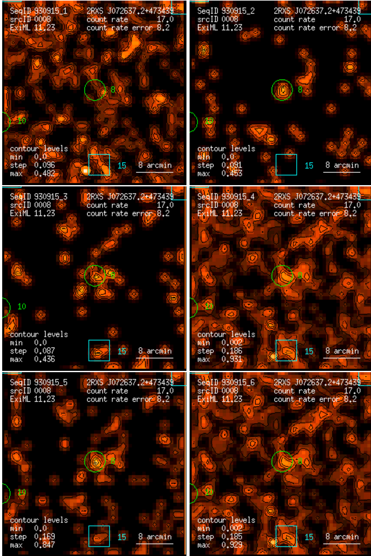
Figure 8: RASS 930915: detection 0008: band rate images, Gaussian filter: (1) PSPC channels 11 – 41, (2) 52 – 90, (3) 91 – 201, (4) 11 – 235, (5) 52 – 201, (6) 11 – 201. Broad band rates in counts/ks. Band rate contour levels in counts/ks/arcmin 2 .
