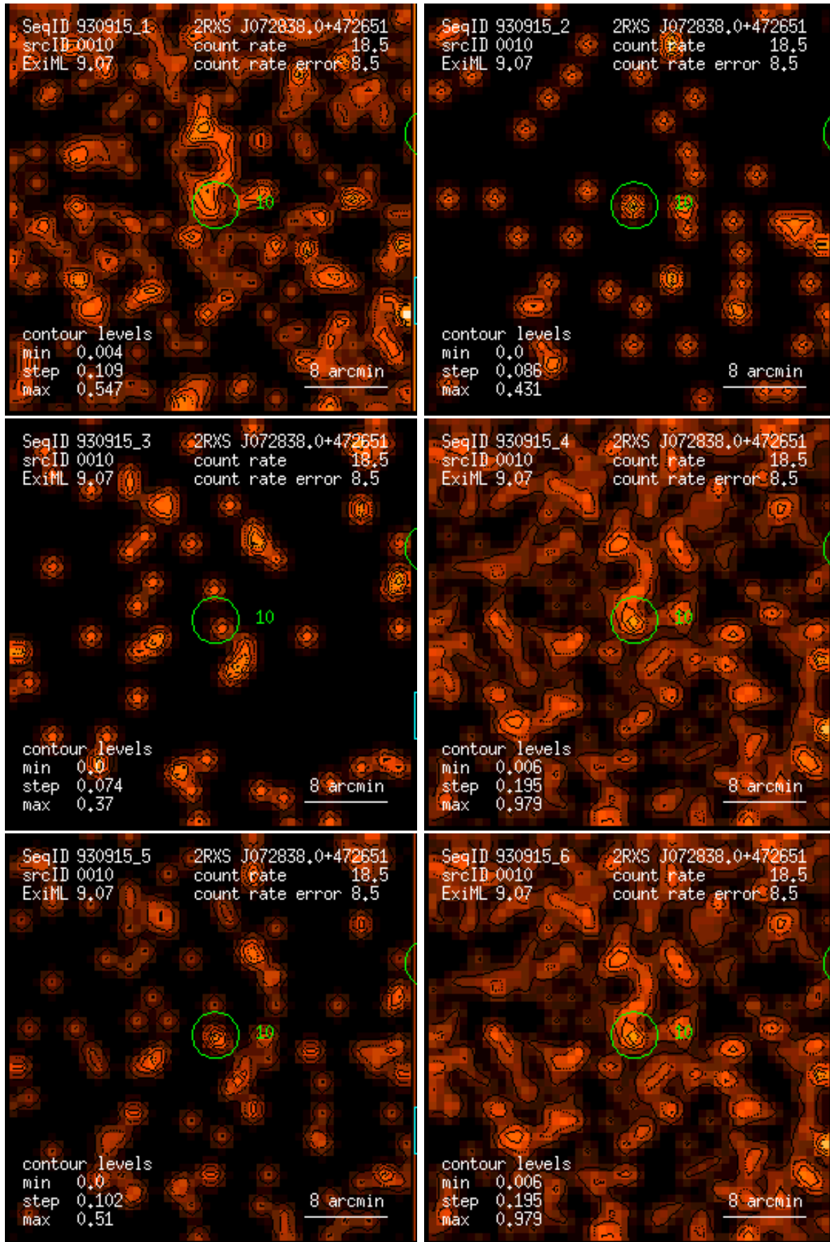
Figure 10: RASS 930915: detection 0010: band rate images, Gaussian filter: (1) PSPC channels 11 – 41, (2) 52 – 90, (3) 91 – 201, (4) 11 – 235, (5) 52 – 201, (6) 11 – 201. Broad band rates in counts/ks. Band rate contour levels in counts/ks/arcmin 2 .
