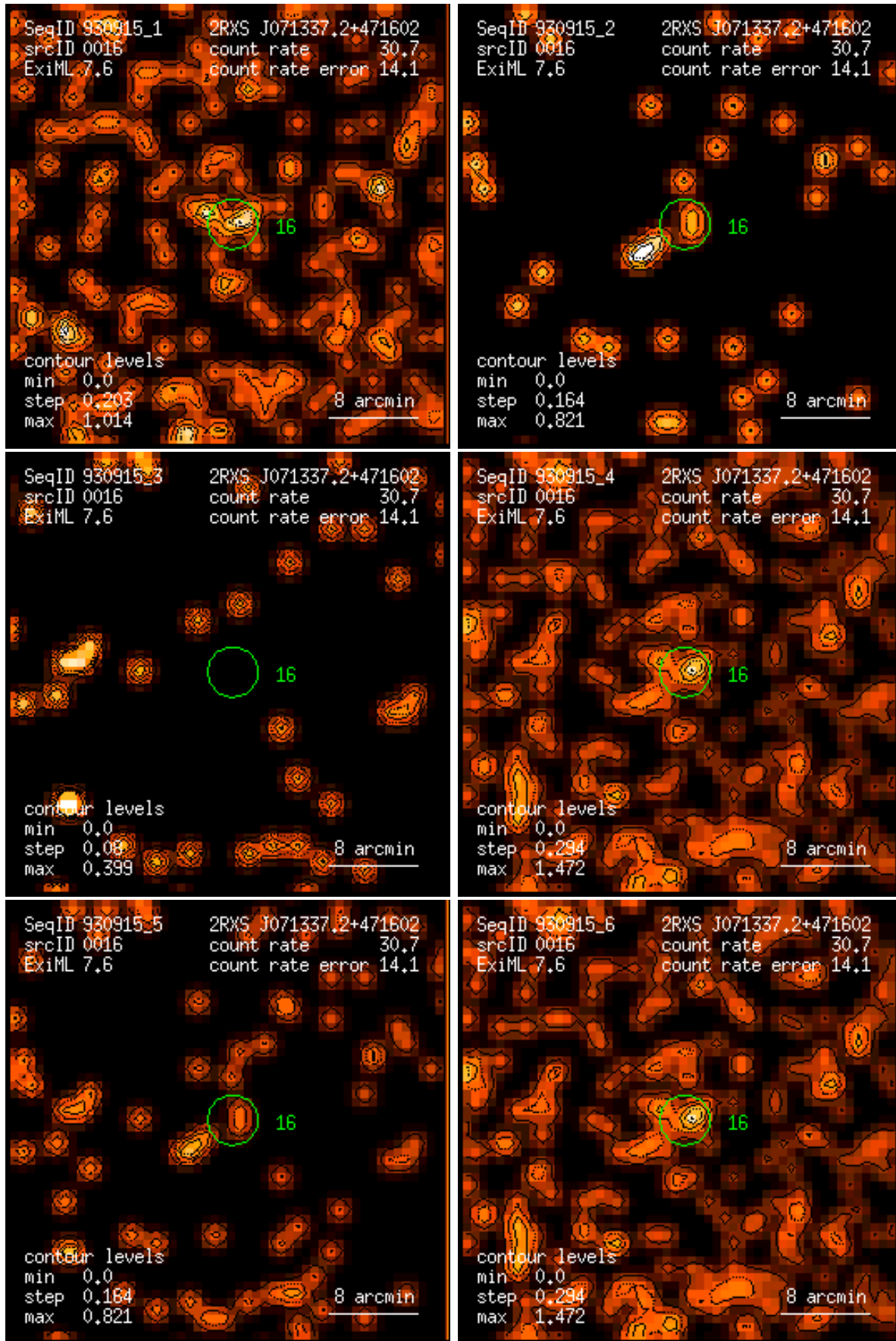
Figure 16: RASS 930915: detection 0016: band rate images, Gaussian filter: (1) PSPC channels 11 – 41, (2) 52 – 90, (3) 91 – 201, (4) 11 – 235, (5) 52 – 201, (6) 11 – 201. Broad band rates in counts/ks. Band rate contour levels in counts/ks/arcmin 2 .
