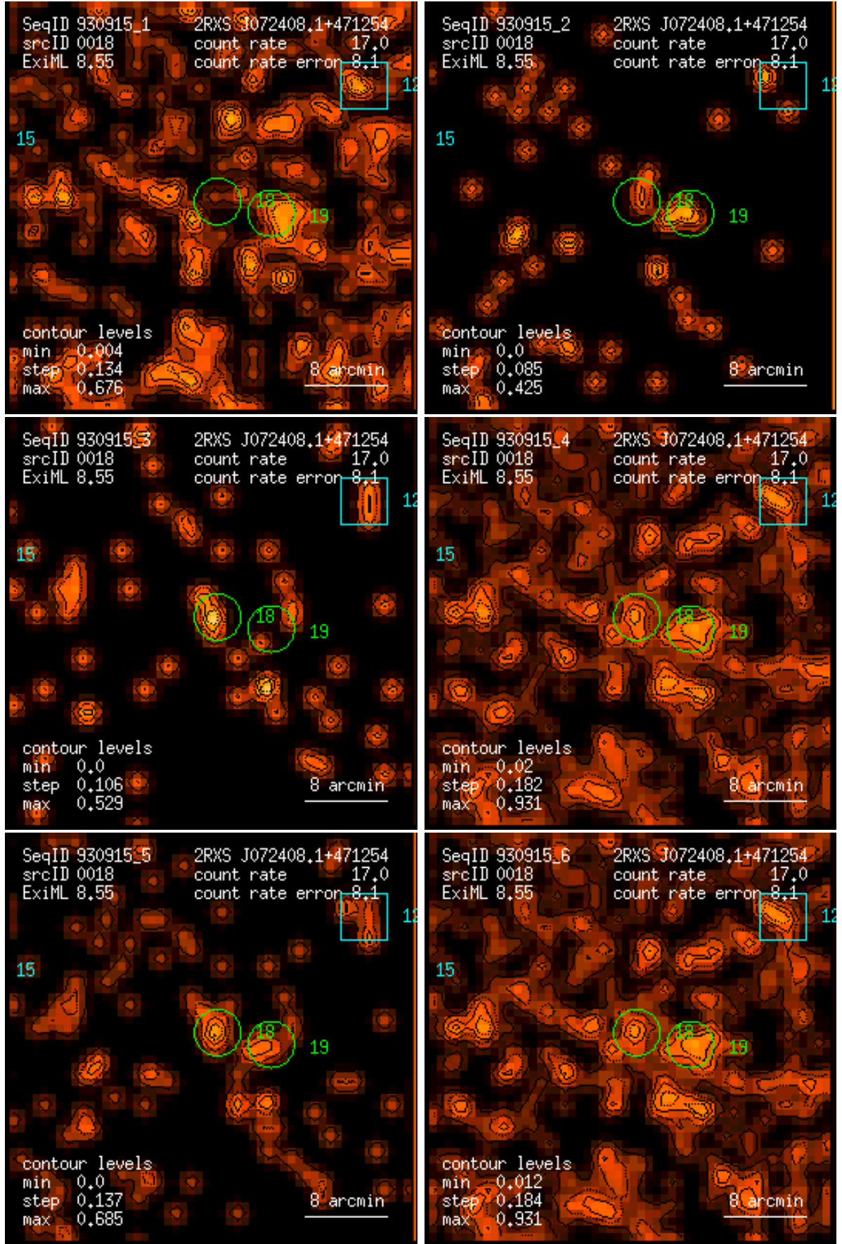
Figure 18: RASS 930915: detection 0018: band rate images, Gaussian filter: (1) PSPC channels 11 – 41, (2) 52 – 90, (3) 91 – 201, (4) 11 – 235, (5) 52 – 201, (6) 11 – 201. Broad band rates in counts/ks. Band rate contour levels in counts/ks/arcmin 2 .
