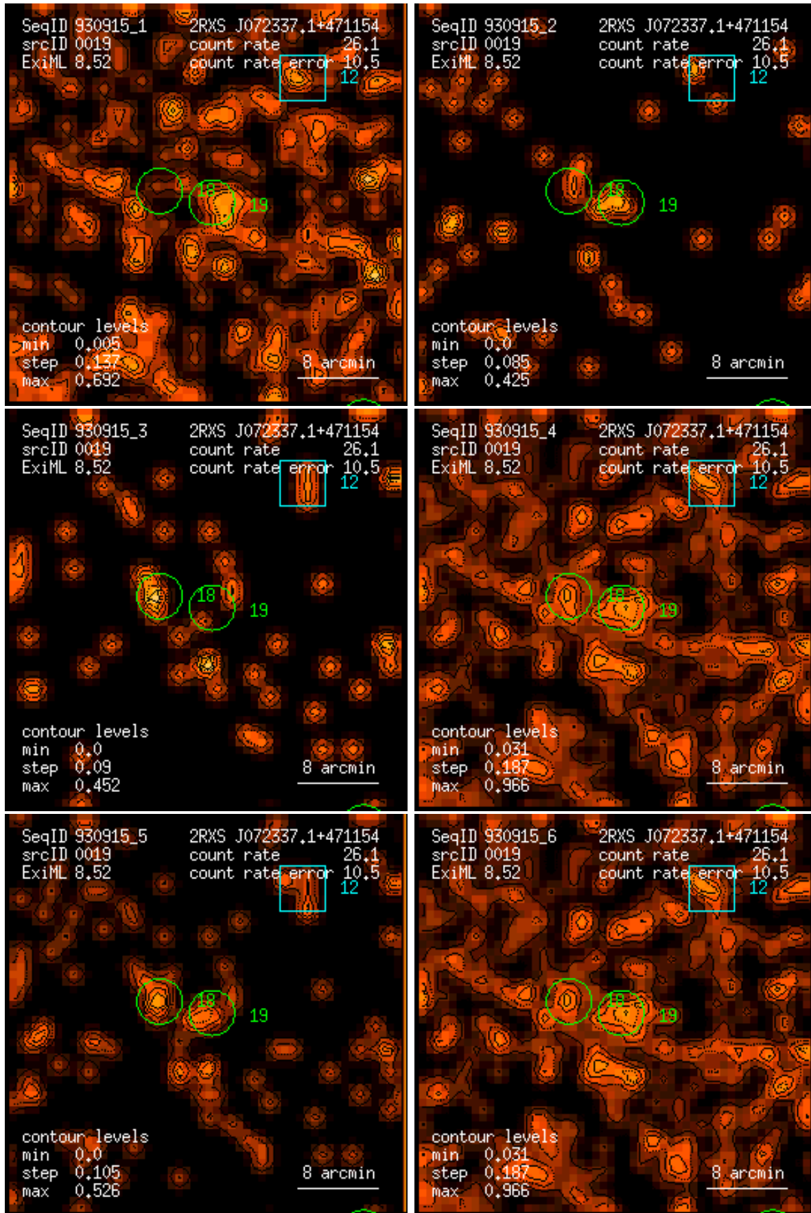
Figure 19: RASS 930915: detection 0019: band rate images, Gaussian filter: (1) PSPC channels 11 – 41, (2) 52 – 90, (3) 91 – 201, (4) 11 – 235, (5) 52 – 201, (6) 11 – 201. Broad band rates in counts/ks. Band rate contour levels in counts/ks/arcmin 2 .
