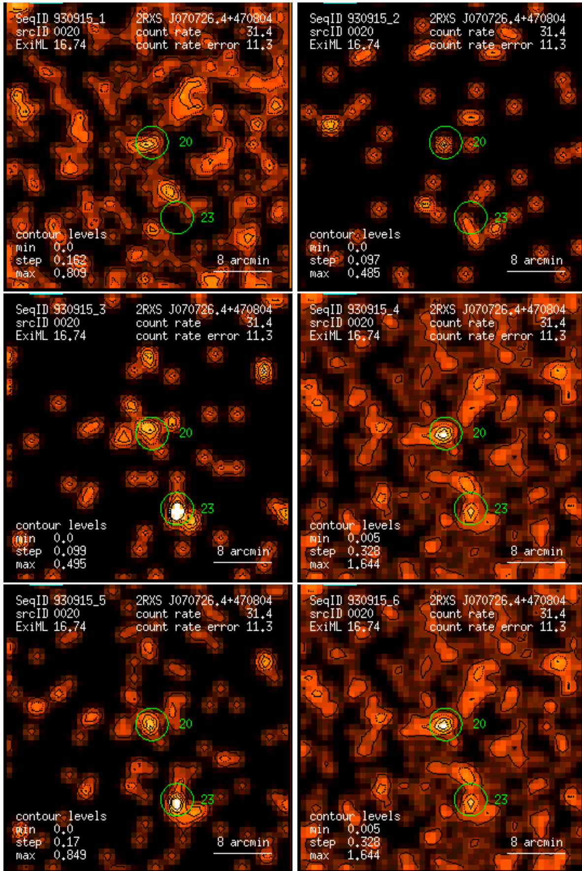
Figure 20: RASS 930915: detection 0020: band rate images, Gaussian filter: (1) PSPC channels 11 – 41, (2) 52 – 90, (3) 91 – 201, (4) 11 – 235, (5) 52 – 201, (6) 11 – 201. Broad band rates in counts/ks. Band rate contour levels in counts/ks/arcmin 2 .
