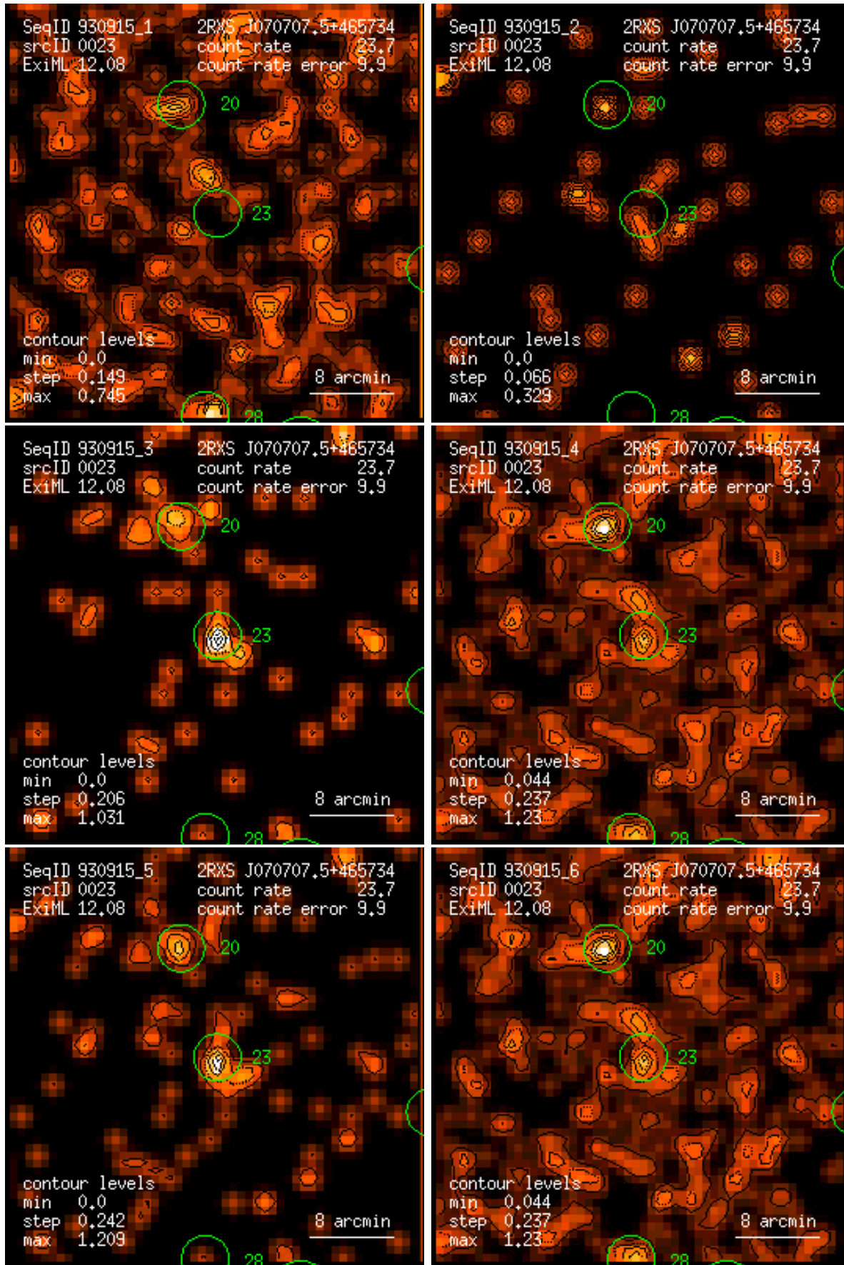
Figure 23: RASS 930915: detection 0023: band rate images, Gaussian filter: (1) PSPC channels 11 – 41, (2) 52 – 90, (3) 91 – 201, (4) 11 – 235, (5) 52 – 201, (6) 11 – 201. Broad band rates in counts/ks. Band rate contour levels in counts/ks/arcmin 2 .
