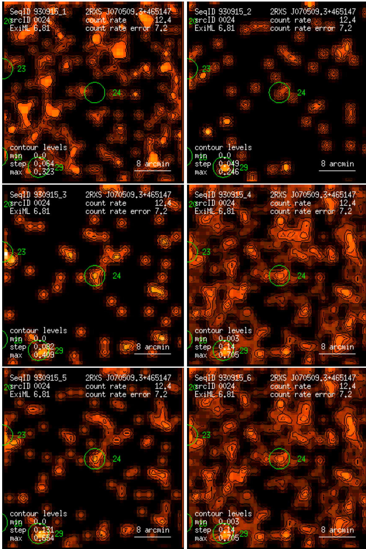
Figure 24: RASS 930915: detection 0024: band rate images, Gaussian filter: (1) PSPC channels 11 – 41, (2) 52 – 90, (3) 91 – 201, (4) 11 – 235, (5) 52 – 201, (6) 11 – 201. Broad band rates in counts/ks. Band rate contour levels in counts/ks/arcmin 2 .
