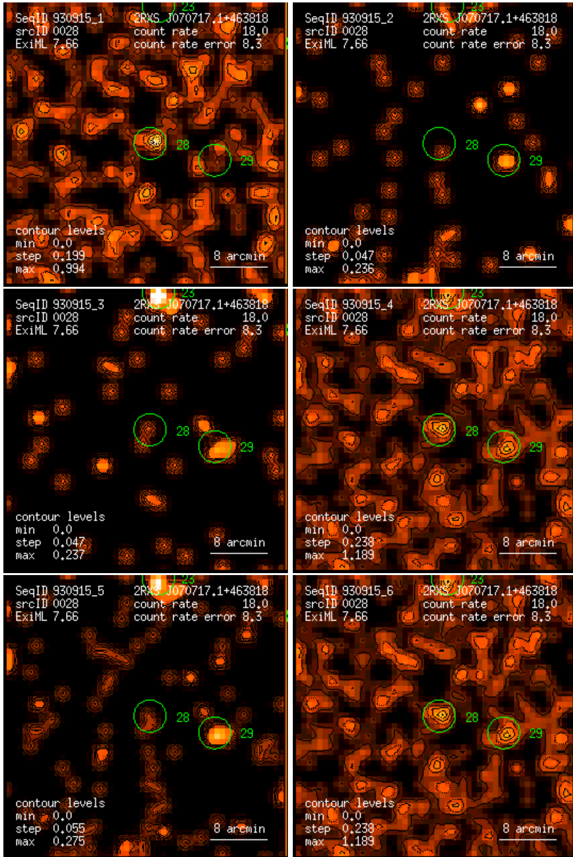
Figure 28: RASS 930915: detection 0028: band rate images, Gaussian filter: (1) PSPC channels 11 – 41, (2) 52 – 90, (3) 91 – 201, (4) 11 – 235, (5) 52 – 201, (6) 11 – 201. Broad band rates in counts/ks. Band rate contour levels in counts/ks/arcmin 2 .
