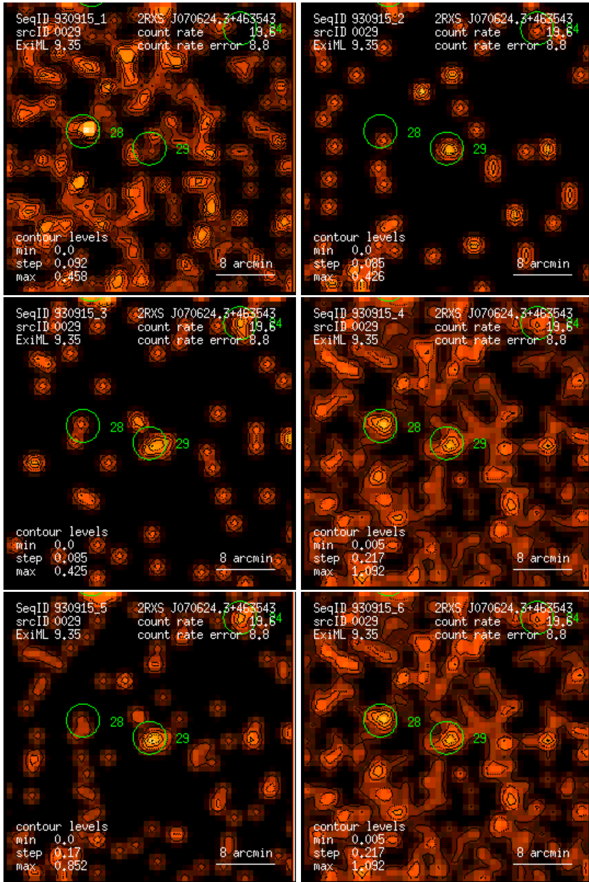
Figure 29: RASS 930915: detection 0029: band rate images, Gaussian filter: (1) PSPC channels 11 – 41, (2) 52 – 90, (3) 91 – 201, (4) 11 – 235, (5) 52 – 201, (6) 11 – 201. Broad band rates in counts/ks. Band rate contour levels in counts/ks/arcmin 2 .
