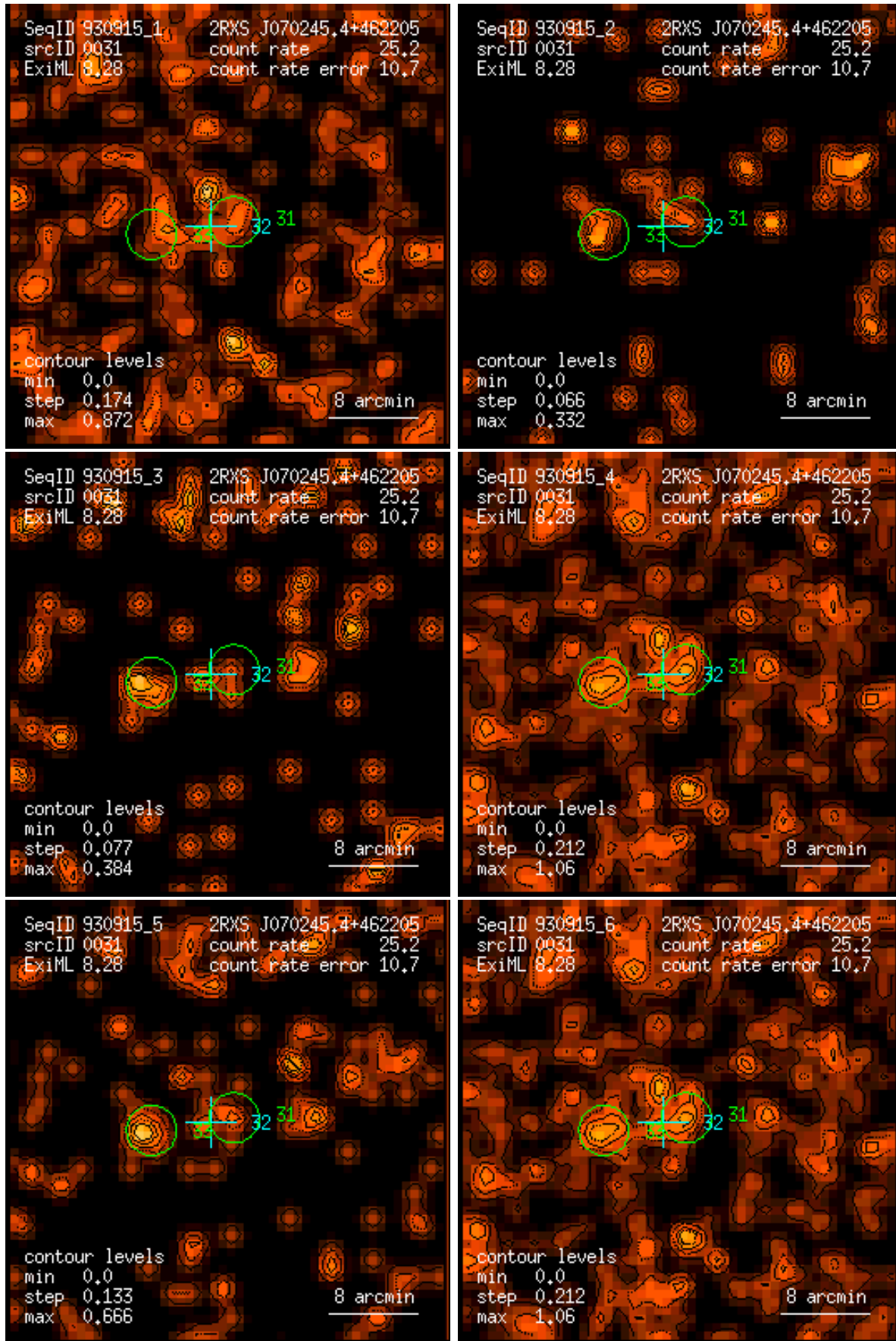
Figure 31: RASS 930915: detection 0031: band rate images, Gaussian filter: (1) PSPC channels 11 – 41, (2) 52 – 90, (3) 91 – 201, (4) 11 – 235, (5) 52 – 201, (6) 11 – 201. Broad band rates in counts/ks. Band rate contour levels in counts/ks/arcmin 2 .
