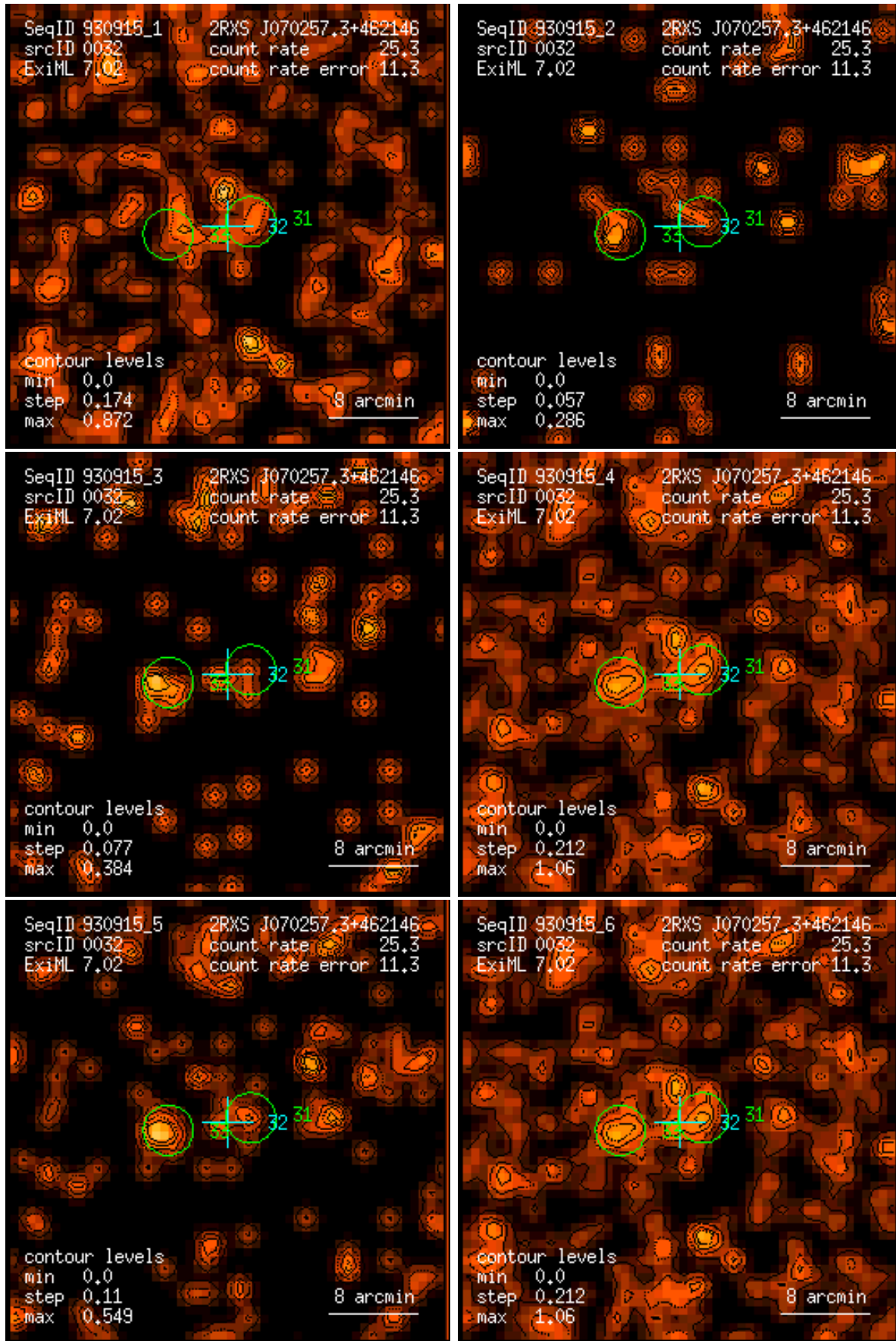
Figure 32: RASS 930915: detection 0032: band rate images, Gaussian filter: (1) PSPC channels 11 – 41, (2) 52 – 90, (3) 91 – 201, (4) 11 – 235, (5) 52 – 201, (6) 11 – 201. Broad band rates in counts/ks. Band rate contour levels in counts/ks/arcmin 2 .
