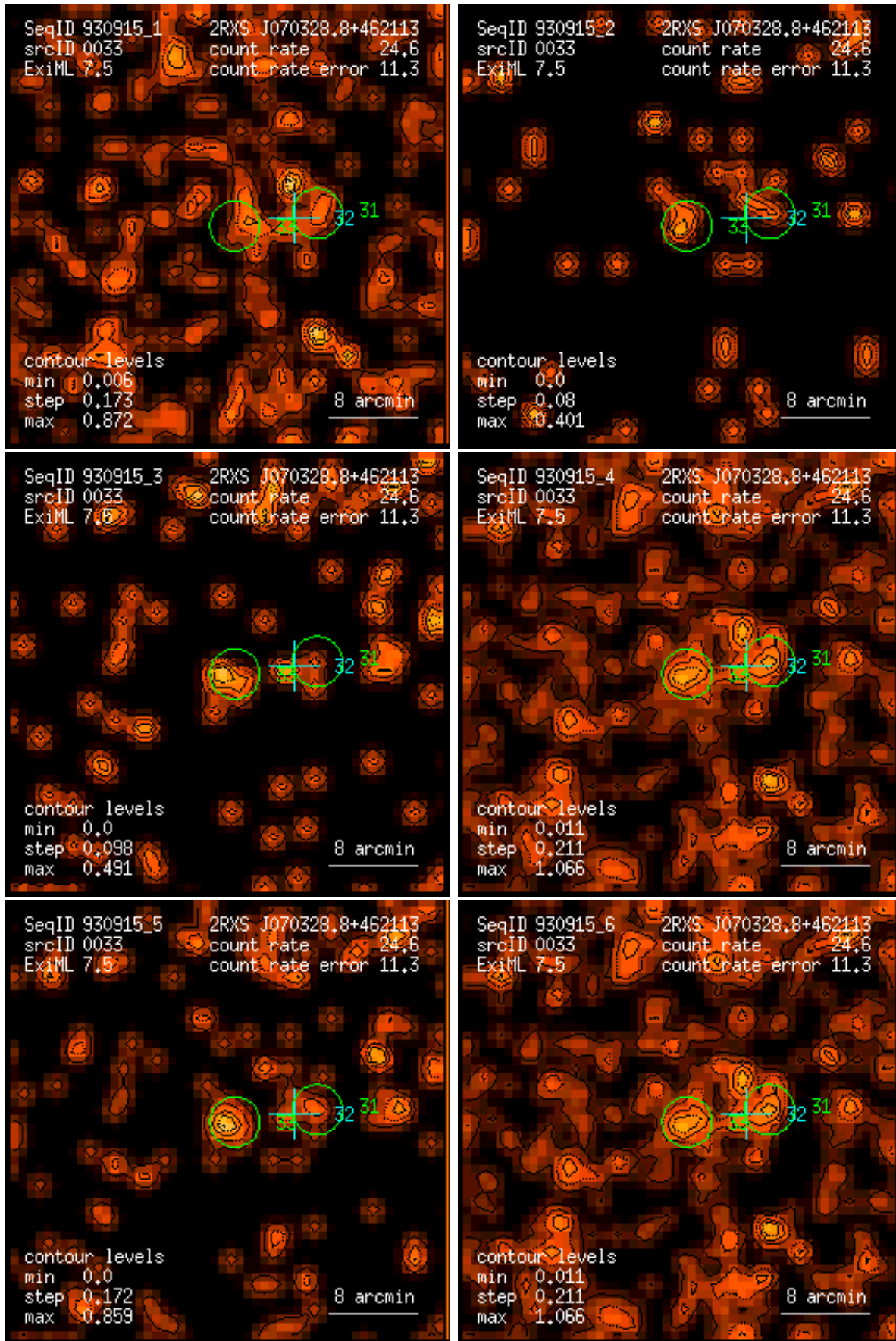
Figure 33: RASS 930915: detection 0033: band rate images, Gaussian filter: (1) PSPC channels 11 – 41, (2) 52 – 90, (3) 91 – 201, (4) 11 – 235, (5) 52 – 201, (6) 11 – 201. Broad band rates in counts/ks. Band rate contour levels in counts/ks/arcmin 2 .
