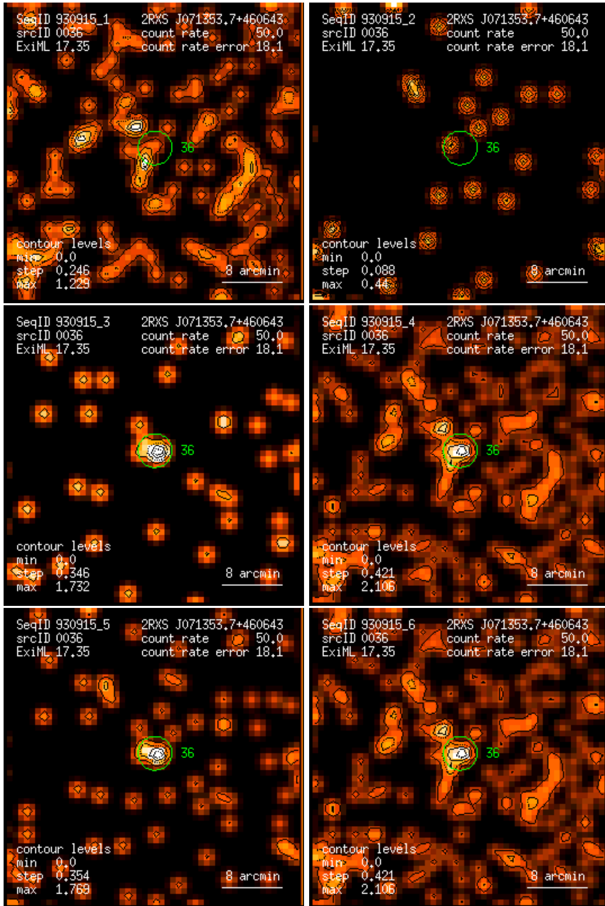
Figure 36: RASS 930915: detection 0036: band rate images, Gaussian filter: (1) PSPC channels 11 – 41, (2) 52 – 90, (3) 91 – 201, (4) 11 – 235, (5) 52 – 201, (6) 11 – 201. Broad band rates in counts/ks. Band rate contour levels in counts/ks/arcmin 2 .
