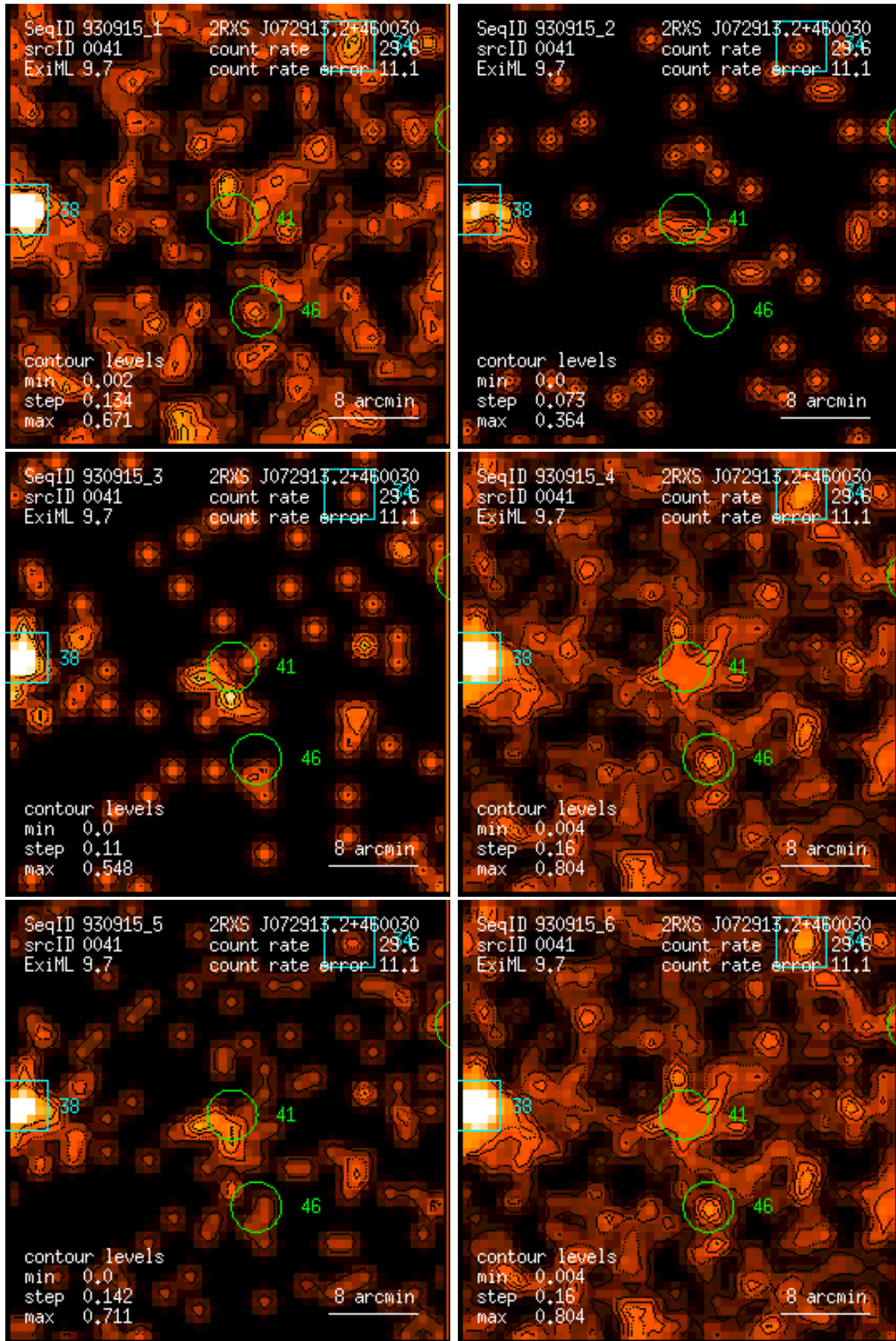
Figure 41: RASS 930915: detection 0041: band rate images, Gaussian filter: (1) PSPC channels 11 – 41, (2) 52 – 90, (3) 91 – 201, (4) 11 – 235, (5) 52 – 201, (6) 11 – 201. Broad band rates in counts/ks. Band rate contour levels in counts/ks/arcmin 2 .
