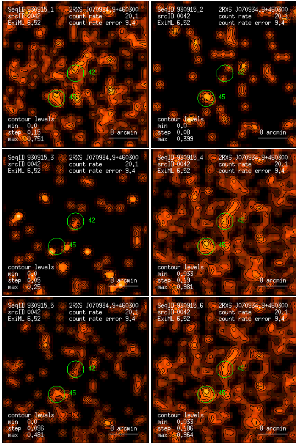
Figure 42: RASS 930915: detection 0042: band rate images, Gaussian filter: (1) PSPC channels 11 – 41, (2) 52 – 90, (3) 91 – 201, (4) 11 – 235, (5) 52 – 201, (6) 11 – 201. Broad band rates in counts/ks. Band rate contour levels in counts/ks/arcmin 2 .
