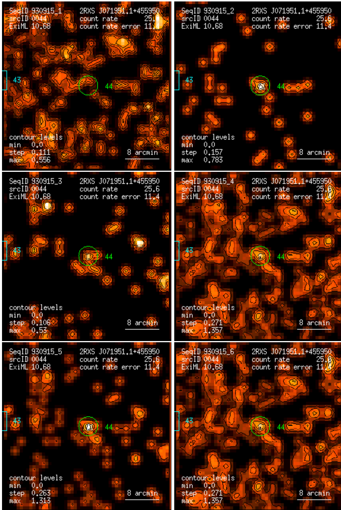
Figure 44: RASS 930915: detection 0044: band rate images, Gaussian filter: (1) PSPC channels 11 – 41, (2) 52 – 90, (3) 91 – 201, (4) 11 – 235, (5) 52 – 201, (6) 11 – 201. Broad band rates in counts/ks. Band rate contour levels in counts/ks/arcmin 2 .
