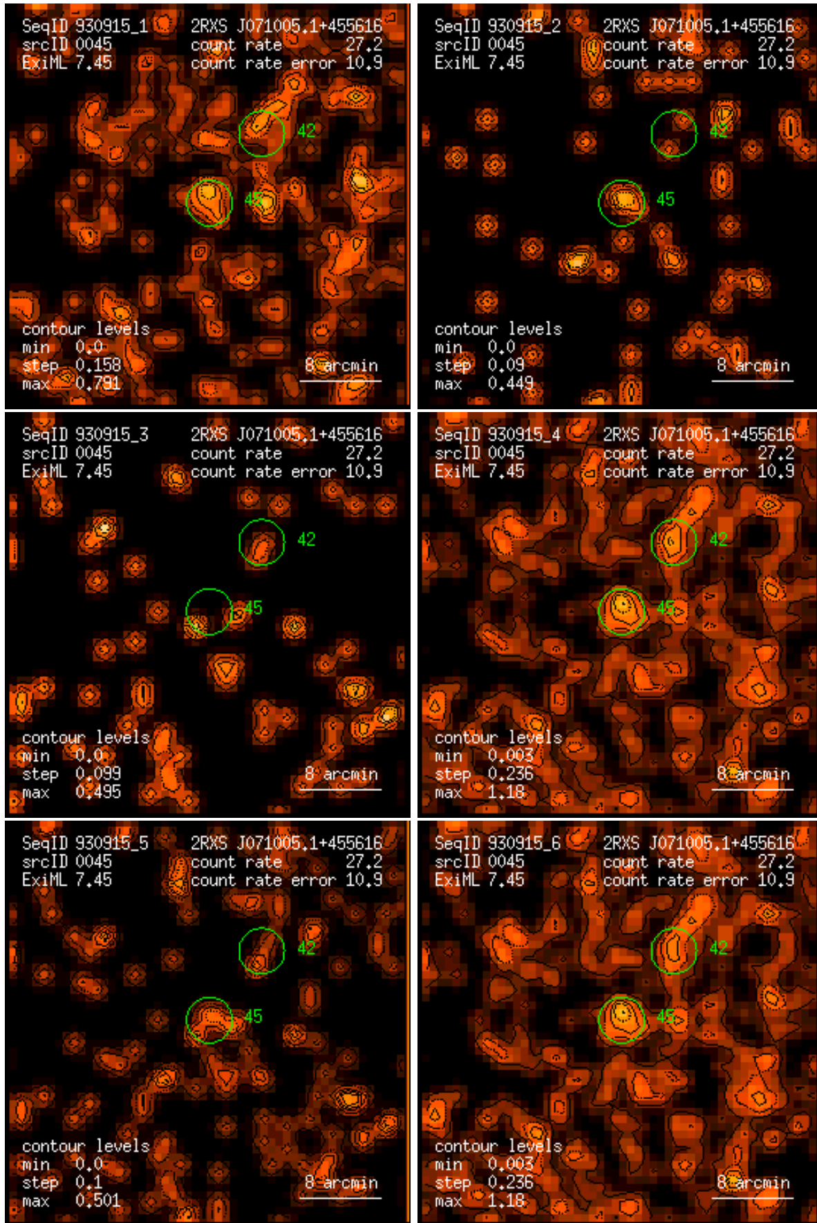
Figure 45: RASS 930915: detection 0045: band rate images, Gaussian filter: (1) PSPC channels 11 – 41, (2) 52 – 90, (3) 91 – 201, (4) 11 – 235, (5) 52 – 201, (6) 11 – 201. Broad band rates in counts/ks. Band rate contour levels in counts/ks/arcmin 2 .
