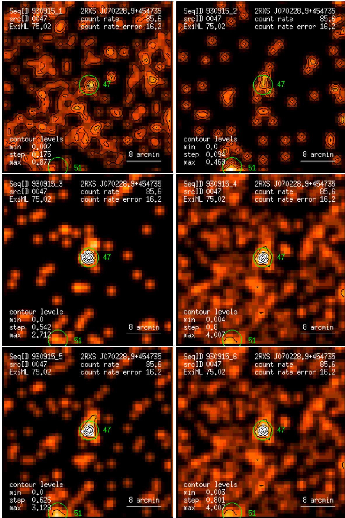
Figure 47: RASS 930915: detection 0047: band rate images, Gaussian filter: (1) PSPC channels 11 – 41, (2) 52 – 90, (3) 91 – 201, (4) 11 – 235, (5) 52 – 201, (6) 11 – 201. Broad band rates in counts/ks. Band rate contour levels in counts/ks/arcmin 2 .
