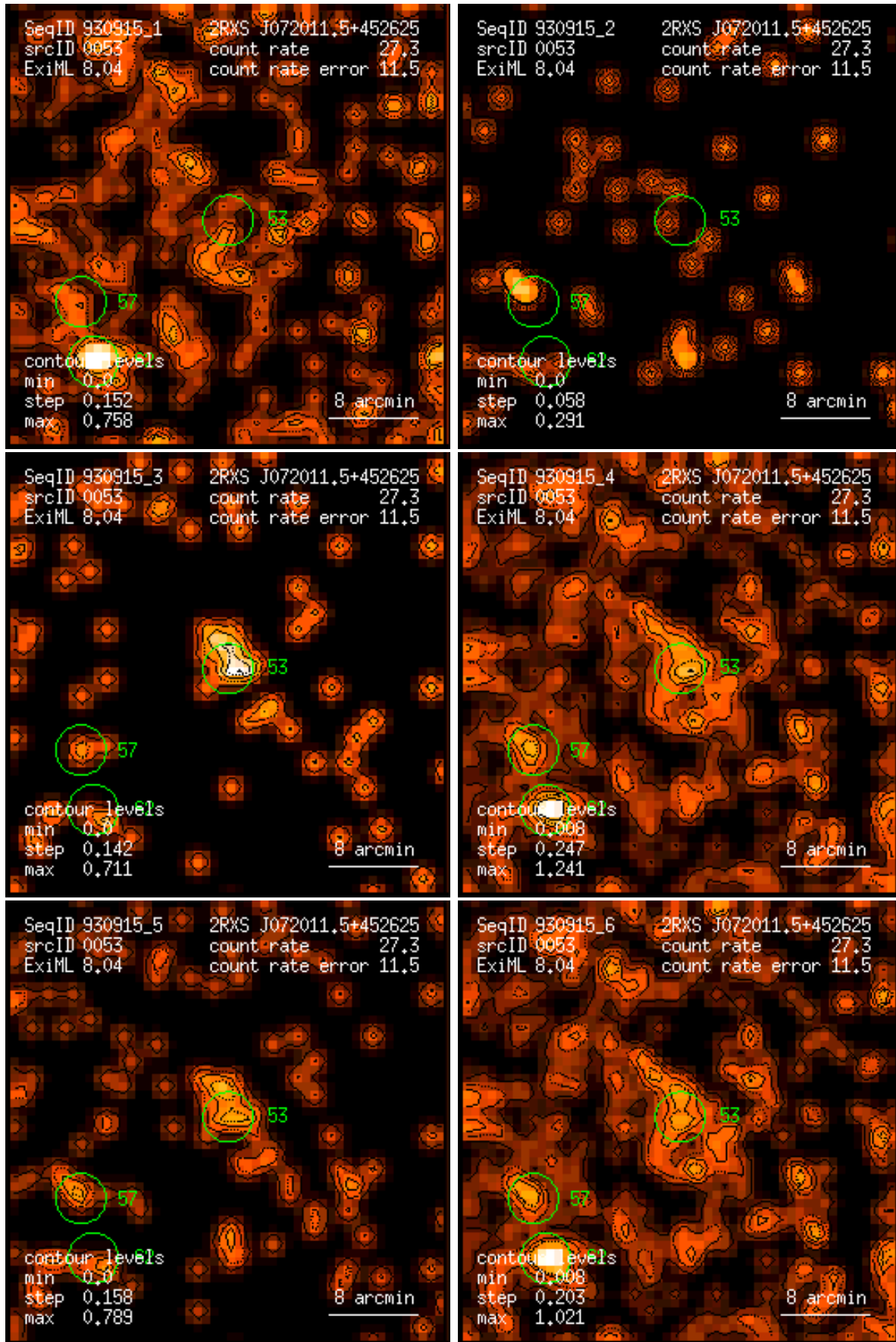
Figure 53: RASS 930915: detection 0053: band rate images, Gaussian filter: (1) PSPC channels 11 – 41, (2) 52 – 90, (3) 91 – 201, (4) 11 – 235, (5) 52 – 201, (6) 11 – 201. Broad band rates in counts/ks. Band rate contour levels in counts/ks/arcmin 2 .
