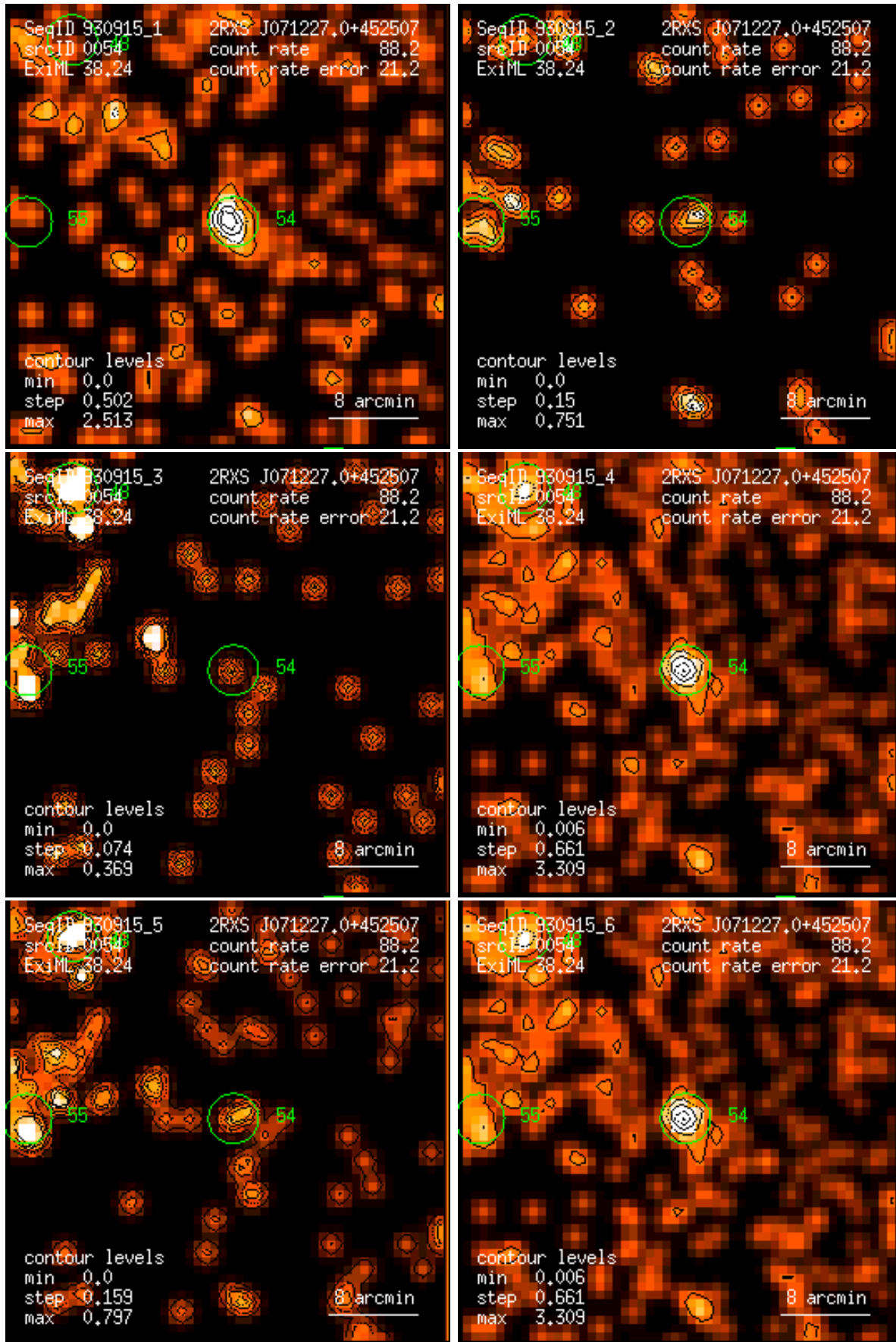
Figure 54: RASS 930915: detection 0054: band rate images, Gaussian filter: (1) PSPC channels 11 – 41, (2) 52 – 90, (3) 91 – 201, (4) 11 – 235, (5) 52 – 201, (6) 11 – 201. Broad band rates in counts/ks. Band rate contour levels in counts/ks/arcmin 2 .
