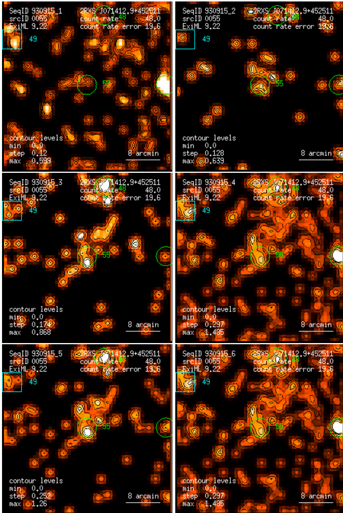
Figure 55: RASS 930915: detection 0055: band rate images, Gaussian filter: (1) PSPC channels 11 – 41, (2) 52 – 90, (3) 91 – 201, (4) 11 – 235, (5) 52 – 201, (6) 11 – 201. Broad band rates in counts/ks. Band rate contour levels in counts/ks/arcmin 2 .
