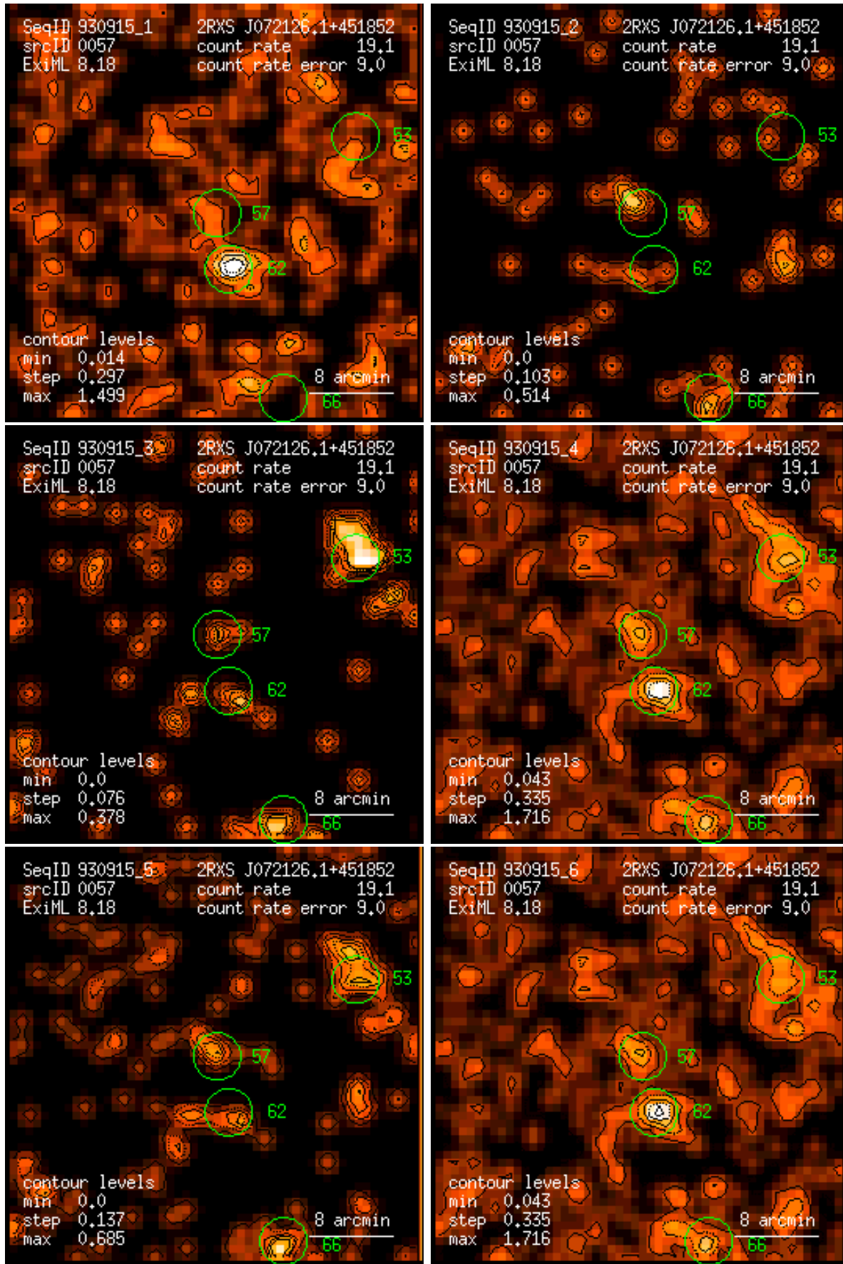
Figure 57: RASS 930915: detection 0057: band rate images, Gaussian filter: (1) PSPC channels 11 – 41, (2) 52 – 90, (3) 91 – 201, (4) 11 – 235, (5) 52 – 201, (6) 11 – 201. Broad band rates in counts/ks. Band rate contour levels in counts/ks/arcmin 2 .
