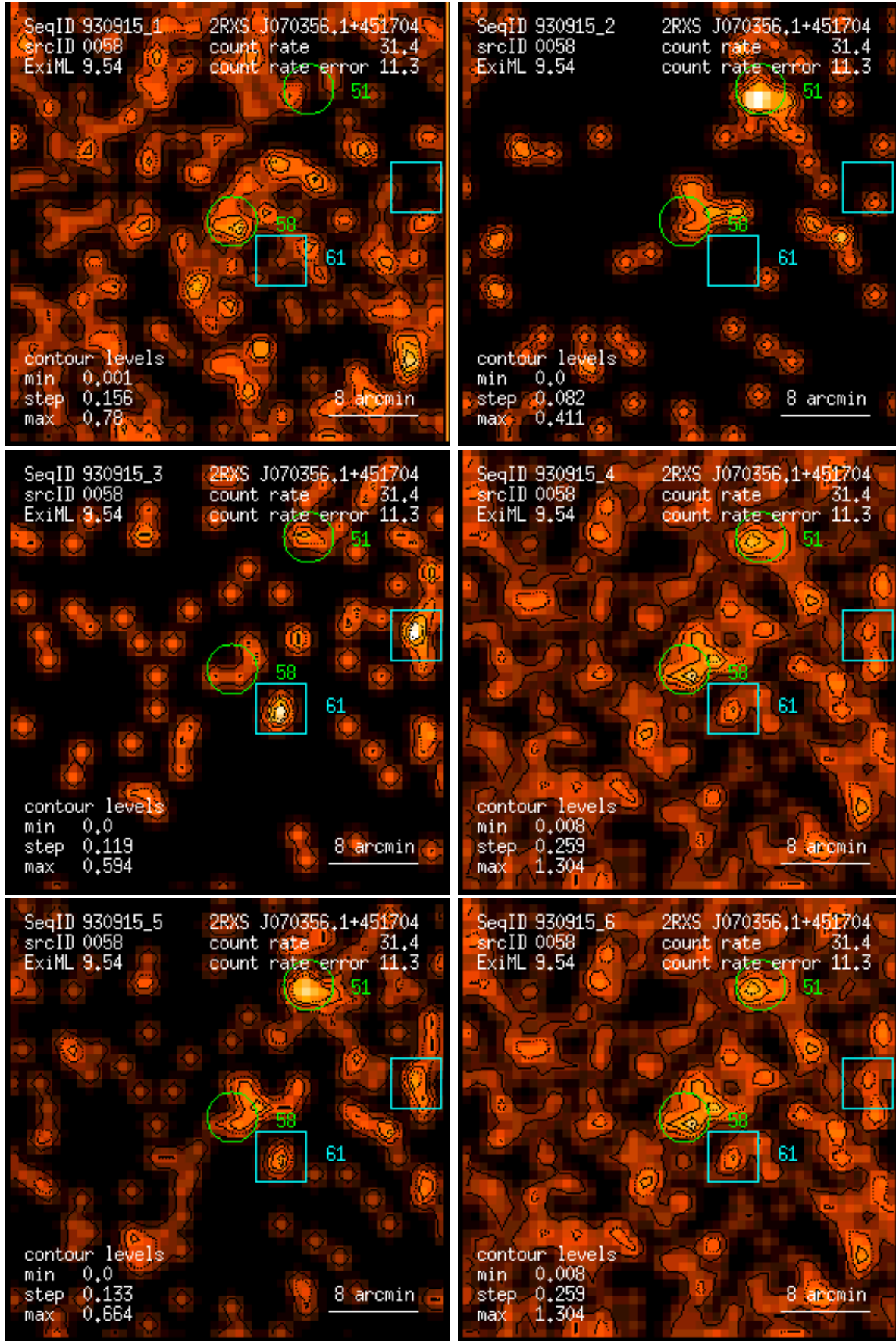
Figure 58: RASS 930915: detection 0058: band rate images, Gaussian filter: (1) PSPC channels 11 – 41, (2) 52 – 90, (3) 91 – 201, (4) 11 – 235, (5) 52 – 201, (6) 11 – 201. Broad band rates in counts/ks. Band rate contour levels in counts/ks/arcmin 2 .
