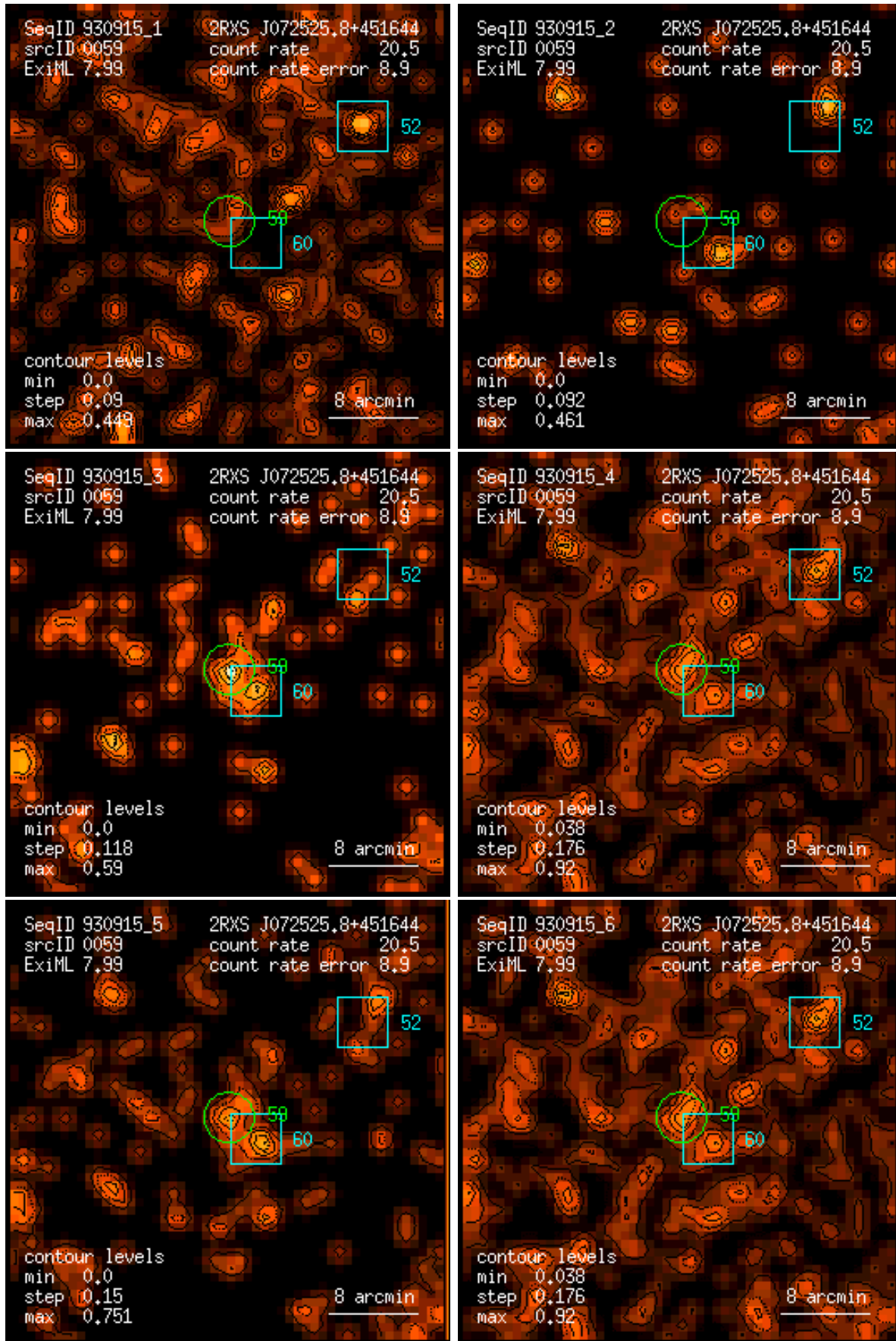
Figure 59: RASS 930915: detection 0059: band rate images, Gaussian filter: (1) PSPC channels 11 – 41, (2) 52 – 90, (3) 91 – 201, (4) 11 – 235, (5) 52 – 201, (6) 11 – 201. Broad band rates in counts/ks. Band rate contour levels in counts/ks/arcmin 2 .
