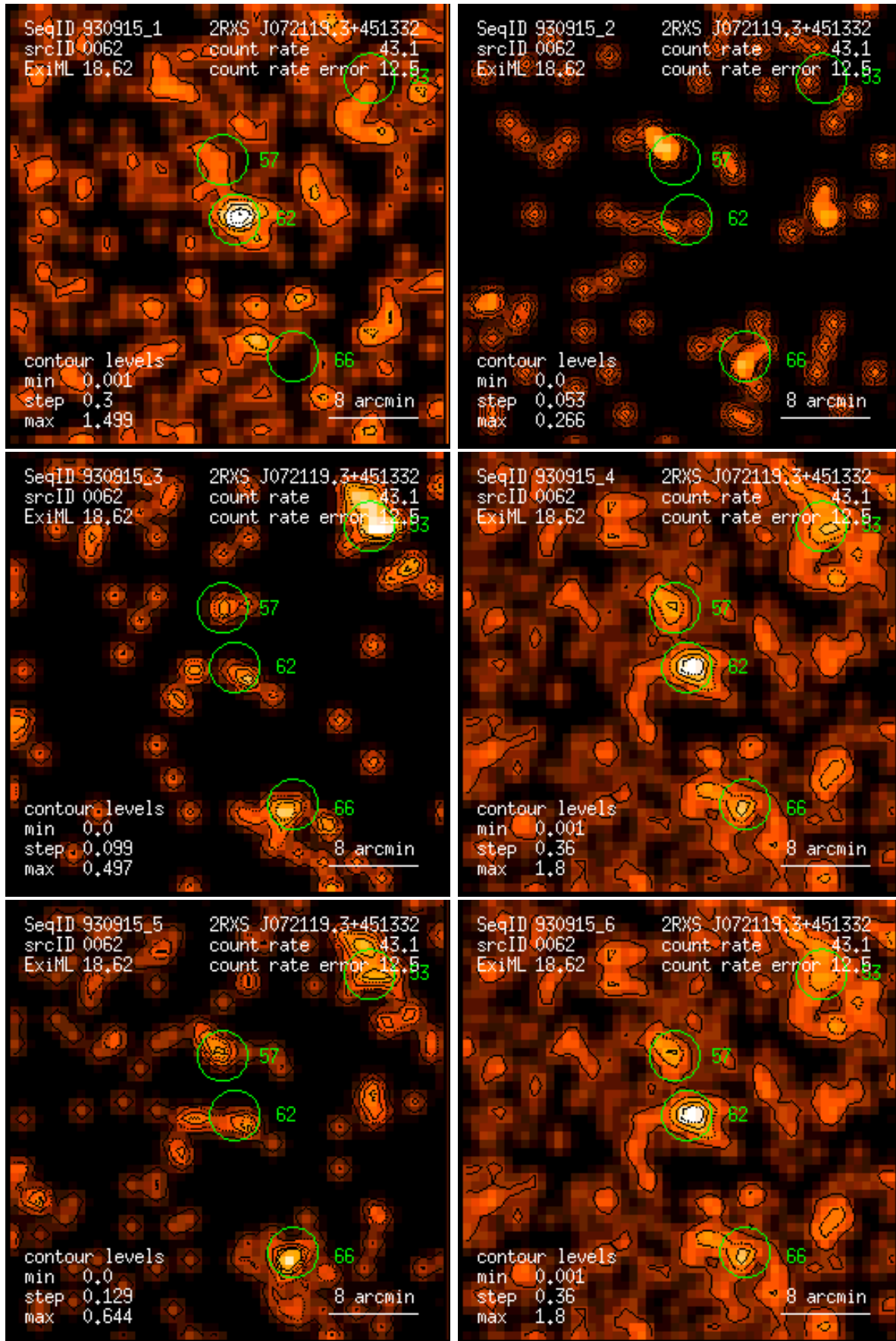
Figure 62: RASS 930915: detection 0062: band rate images, Gaussian filter: (1) PSPC channels 11 – 41, (2) 52 – 90, (3) 91 – 201, (4) 11 – 235, (5) 52 – 201, (6) 11 – 201. Broad band rates in counts/ks. Band rate contour levels in counts/ks/arcmin 2 .
