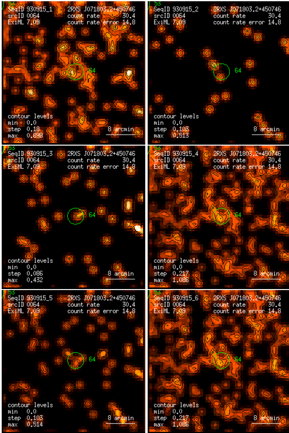
Figure 64: RASS 930915: detection 0064: band rate images, Gaussian filter: (1) PSPC channels 11 – 41, (2) 52 – 90, (3) 91 – 201, (4) 11 – 235, (5) 52 – 201, (6) 11 – 201. Broad band rates in counts/ks. Band rate contour levels in counts/ks/arcmin 2 .
