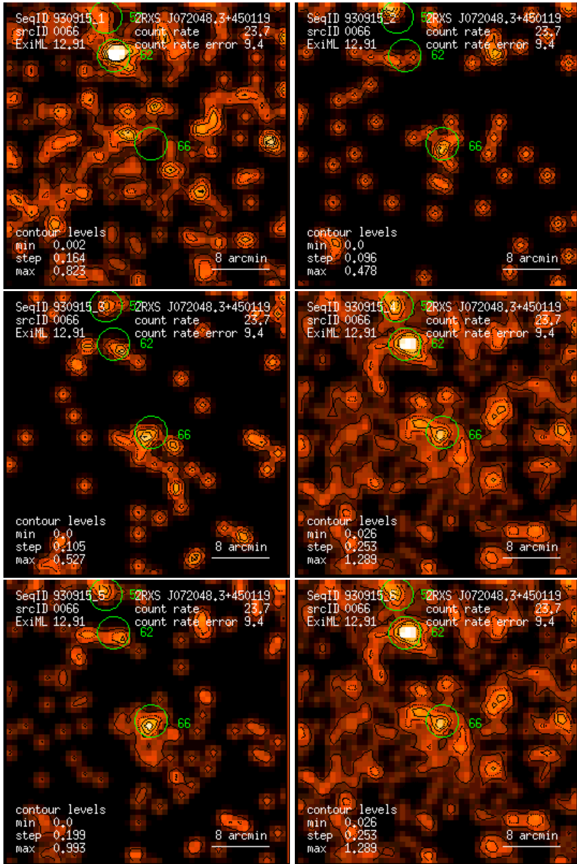
Figure 66: RASS 930915: detection 0066: band rate images, Gaussian filter: (1) PSPC channels 11 – 41, (2) 52 – 90, (3) 91 – 201, (4) 11 – 235, (5) 52 – 201, (6) 11 – 201. Broad band rates in counts/ks. Band rate contour levels in counts/ks/arcmin 2 .
