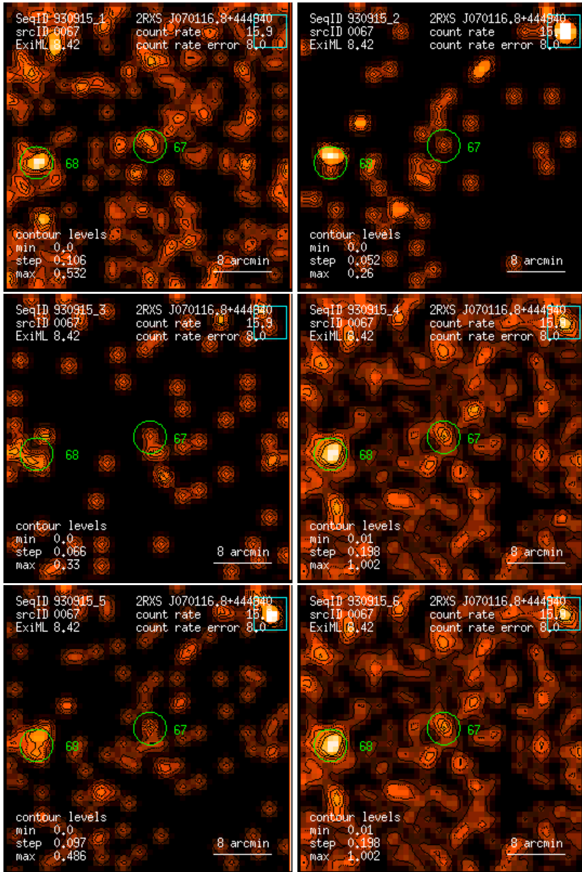
Figure 67: RASS 930915: detection 0067: band rate images, Gaussian filter: (1) PSPC channels 11 – 41, (2) 52 – 90, (3) 91 – 201, (4) 11 – 235, (5) 52 – 201, (6) 11 – 201. Broad band rates in counts/ks. Band rate contour levels in counts/ks/arcmin 2 .
