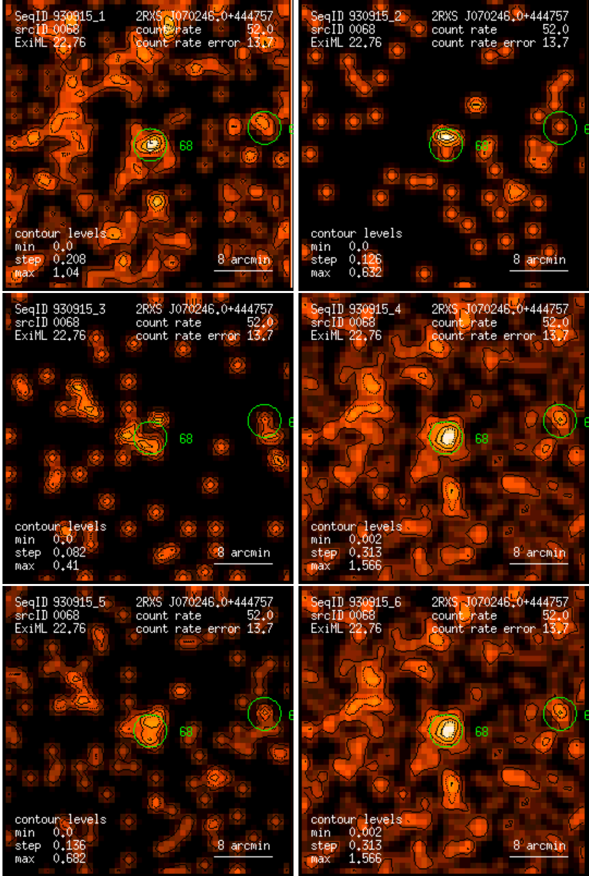
Figure 68: RASS 930915: detection 0068: band rate images, Gaussian filter: (1) PSPC channels 11 – 41, (2) 52 – 90, (3) 91 – 201, (4) 11 – 235, (5) 52 – 201, (6) 11 – 201. Broad band rates in counts/ks. Band rate contour levels in counts/ks/arcmin 2 .
