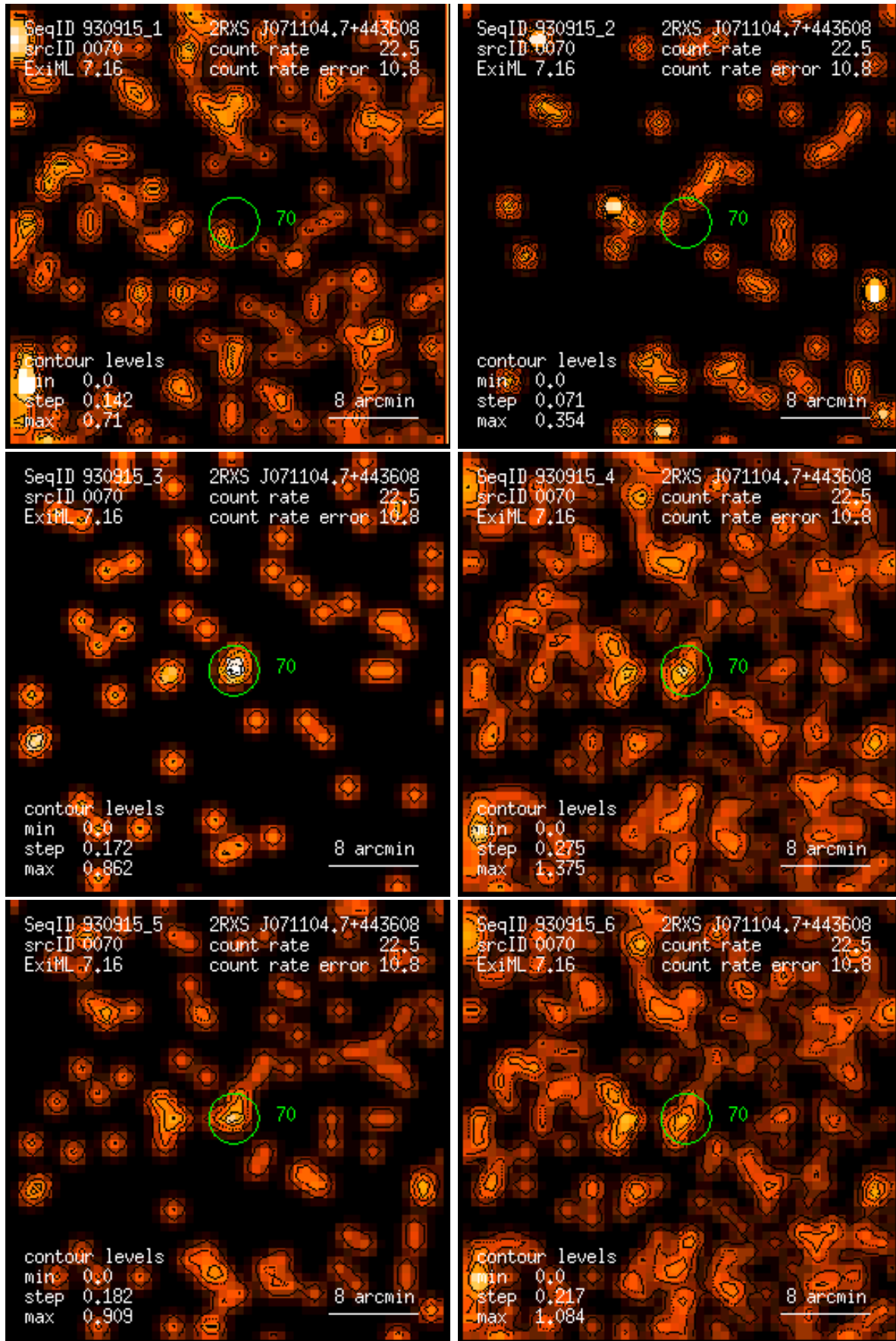
Figure 70: RASS 930915: detection 0070: band rate images, Gaussian filter: (1) PSPC channels 11 – 41, (2) 52 – 90, (3) 91 – 201, (4) 11 – 235, (5) 52 – 201, (6) 11 – 201. Broad band rates in counts/ks. Band rate contour levels in counts/ks/arcmin 2 .
