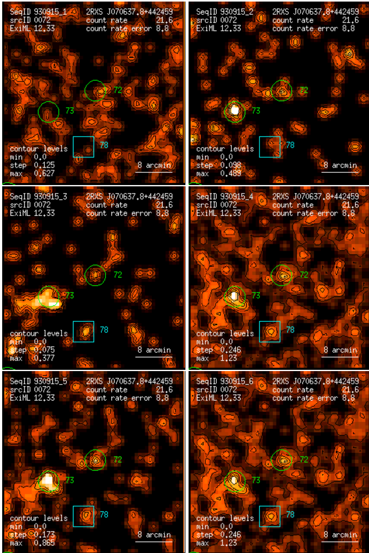
Figure 72: RASS 930915: detection 0072: band rate images, Gaussian filter: (1) PSPC channels 11 – 41, (2) 52 – 90, (3) 91 – 201, (4) 11 – 235, (5) 52 – 201, (6) 11 – 201. Broad band rates in counts/ks. Band rate contour levels in counts/ks/arcmin 2 .
