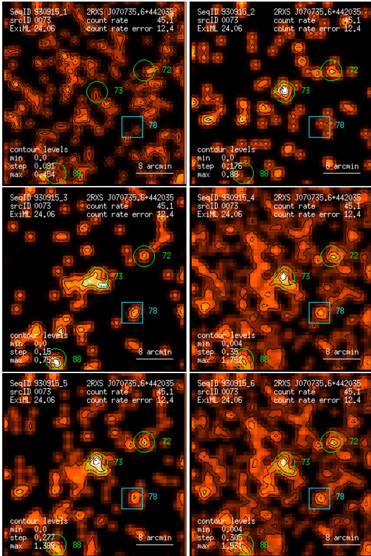
Figure 73: RASS 930915: detection 0073: band rate images, Gaussian filter: (1) PSPC channels 11 – 41, (2) 52 – 90, (3) 91 – 201, (4) 11 – 235, (5) 52 – 201, (6) 11 – 201. Broad band rates in counts/ks. Band rate contour levels in counts/ks/arcmin 2 .
