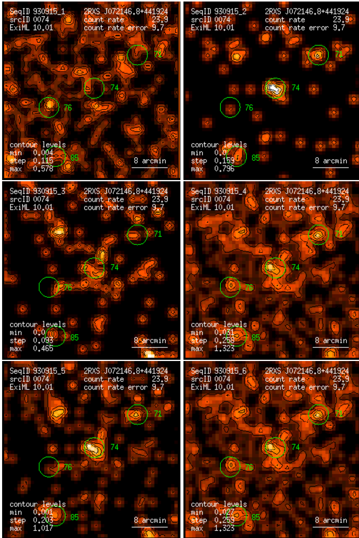
Figure 74: RASS 930915: detection 0074: band rate images, Gaussian filter: (1) PSPC channels 11 – 41, (2) 52 – 90, (3) 91 – 201, (4) 11 – 235, (5) 52 – 201, (6) 11 – 201. Broad band rates in counts/ks. Band rate contour levels in counts/ks/arcmin 2 .
