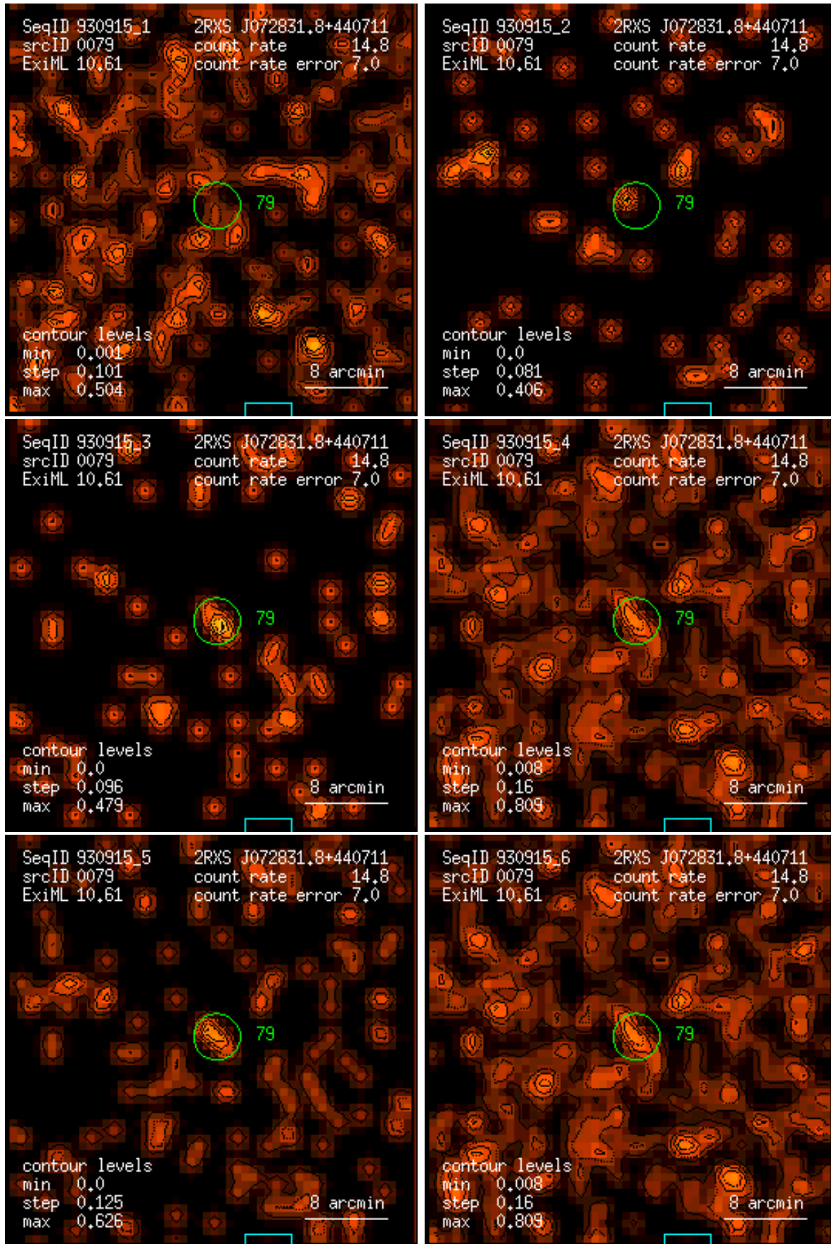
Figure 79: RASS 930915: detection 0079: band rate images, Gaussian filter: (1) PSPC channels 11 – 41, (2) 52 – 90, (3) 91 – 201, (4) 11 – 235, (5) 52 – 201, (6) 11 – 201. Broad band rates in counts/ks. Band rate contour levels in counts/ks/arcmin 2 .
