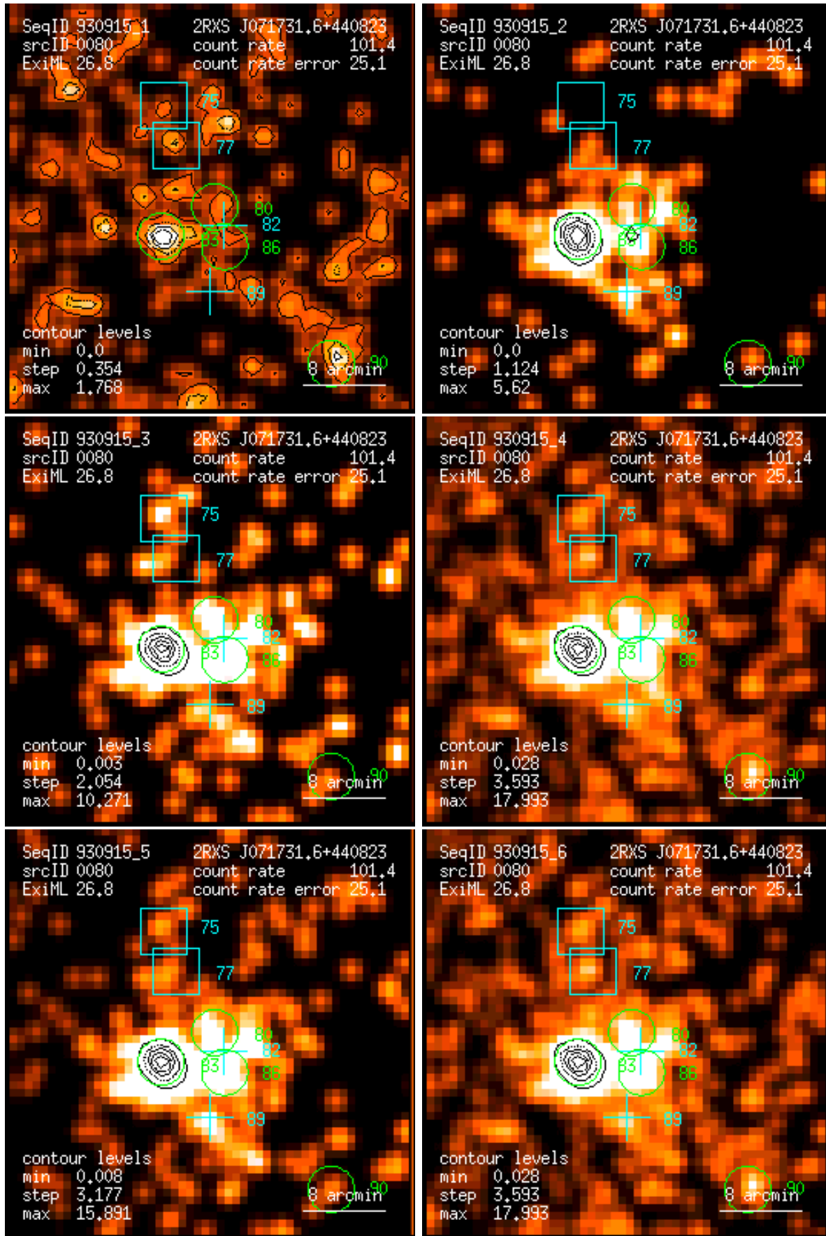
Figure 80: RASS 930915: detection 0080: band rate images, Gaussian filter: (1) PSPC channels 11 – 41, (2) 52 – 90, (3) 91 – 201, (4) 11 – 235, (5) 52 – 201, (6) 11 – 201. Broad band rates in counts/ks. Band rate contour levels in counts/ks/arcmin 2 .
