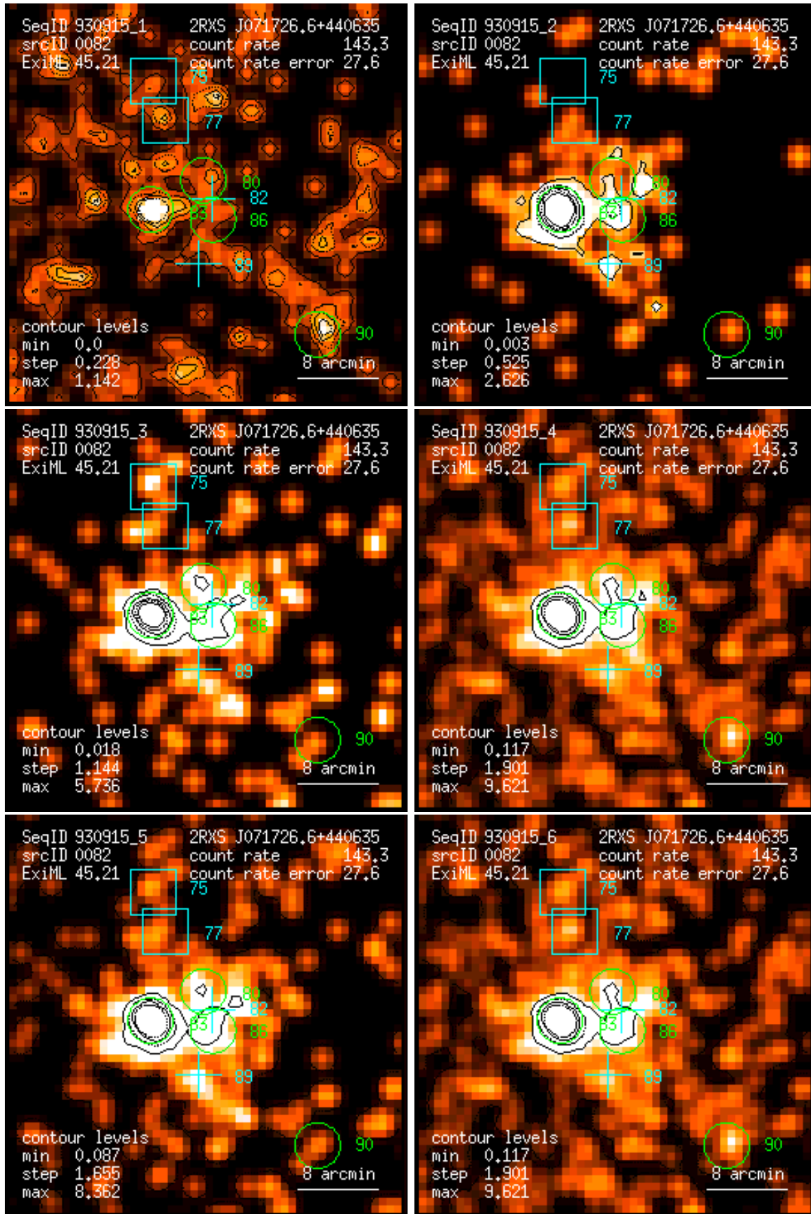
Figure 82: RASS 930915: detection 0082: band rate images, Gaussian filter: (1) PSPC channels 11 – 41, (2) 52 – 90, (3) 91 – 201, (4) 11 – 235, (5) 52 – 201, (6) 11 – 201. Broad band rates in counts/ks. Band rate contour levels in counts/ks/arcmin 2 .
