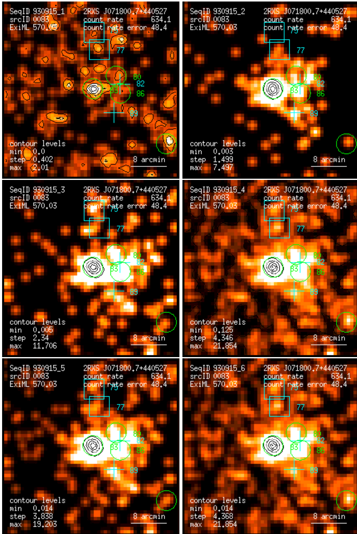
Figure 83: RASS 930915: detection 0083: band rate images, Gaussian filter: (1) PSPC channels 11 – 41, (2) 52 – 90, (3) 91 – 201, (4) 11 – 235, (5) 52 – 201, (6) 11 – 201. Broad band rates in counts/ks. Band rate contour levels in counts/ks/arcmin 2 .
