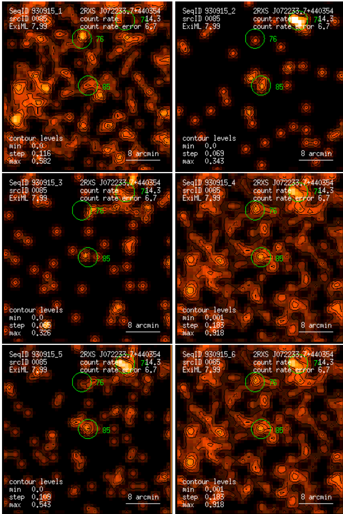
Figure 85: RASS 930915: detection 0085: band rate images, Gaussian filter: (1) PSPC channels 11 – 41, (2) 52 – 90, (3) 91 – 201, (4) 11 – 235, (5) 52 – 201, (6) 11 – 201. Broad band rates in counts/ks. Band rate contour levels in counts/ks/arcmin 2 .
